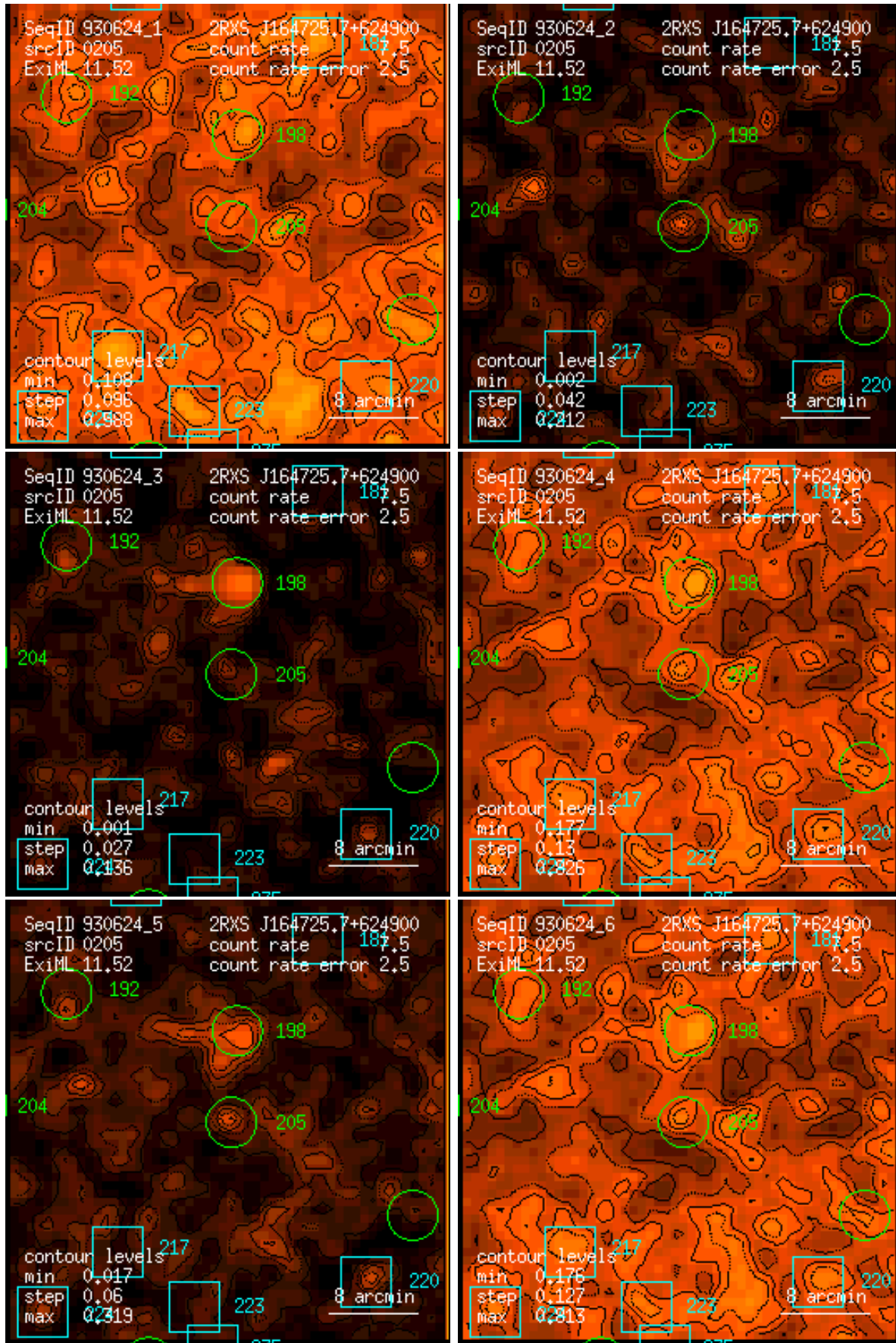
Figure 205: RASS 930624: detection 0205: band rate images, Gaussian filter: (1) PSPC channels 11 – 41, (2) 52 – 90, (3) 91 – 201, (4) 11 – 235, (5) 52 – 201, (6) 11 – 201. Broad band rates in counts/ks. Band rate contour levels in counts/ks/arcmin 2 .
