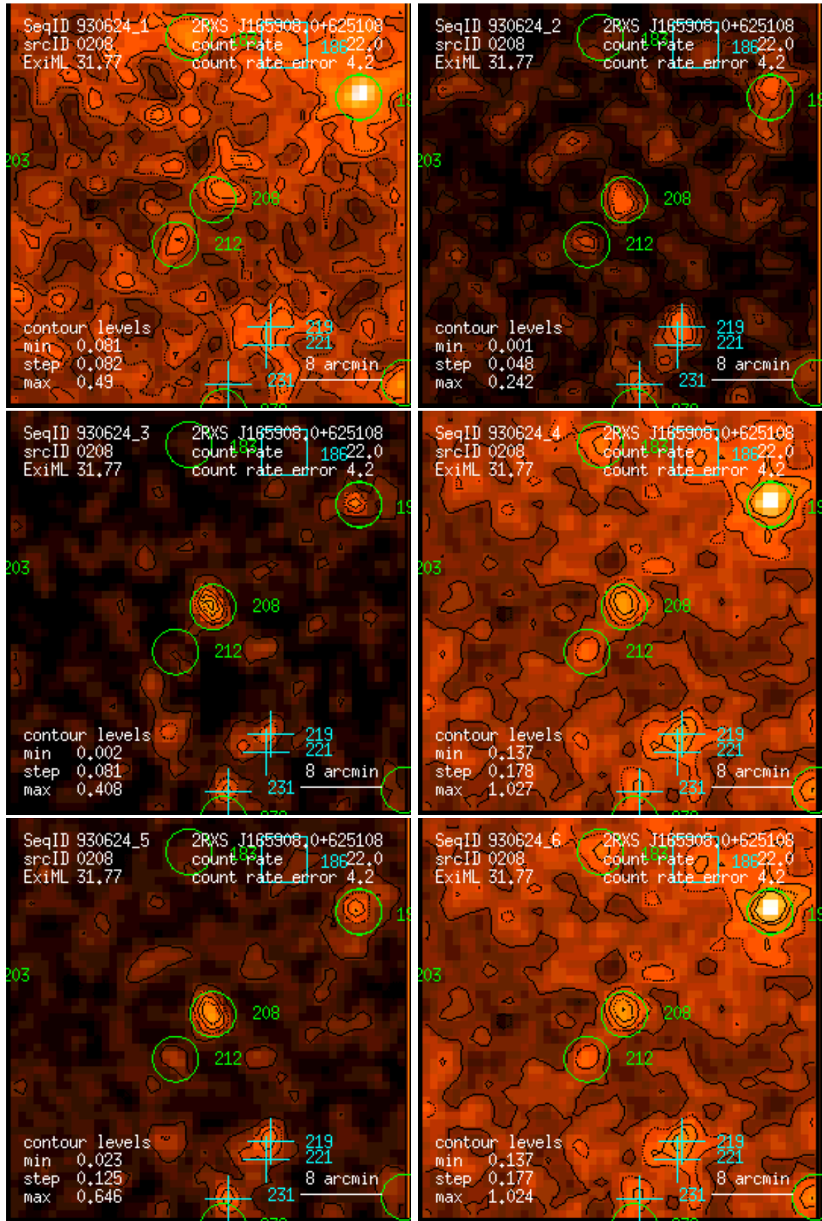
Figure 208: RASS 930624: detection 0208: band rate images, Gaussian filter: (1) PSPC channels 11 – 41, (2) 52 – 90, (3) 91 – 201, (4) 11 – 235, (5) 52 – 201, (6) 11 – 201. Broad band rates in counts/ks. Band rate contour levels in counts/ks/arcmin 2 .
