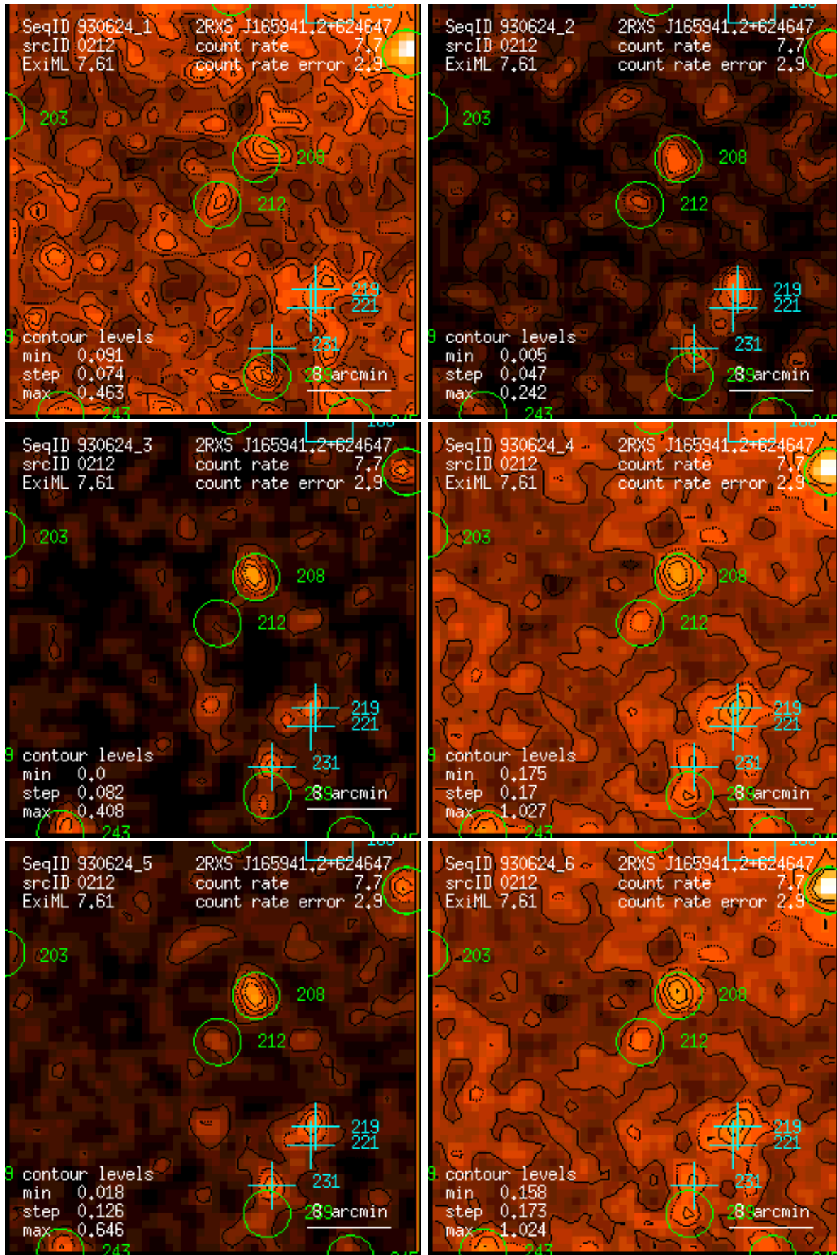
Figure 212: RASS 930624: detection 0212: band rate images, Gaussian filter: (1) PSPC channels 11 – 41, (2) 52 – 90, (3) 91 – 201, (4) 11 – 235, (5) 52 – 201, (6) 11 – 201. Broad band rates in counts/ks. Band rate contour levels in counts/ks/arcmin 2 .
