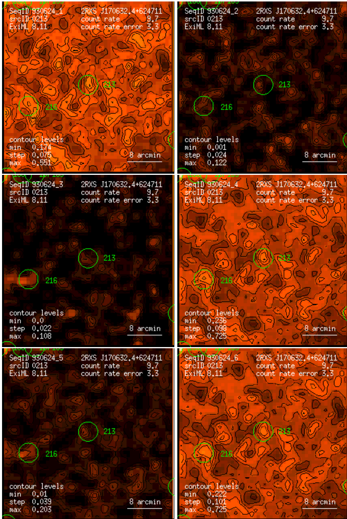
Figure 213: RASS 930624: detection 0213: band rate images, Gaussian filter: (1) PSPC channels 11 – 41, (2) 52 – 90, (3) 91 – 201, (4) 11 – 235, (5) 52 – 201, (6) 11 – 201. Broad band rates in counts/ks. Band rate contour levels in counts/ks/arcmin 2 .
