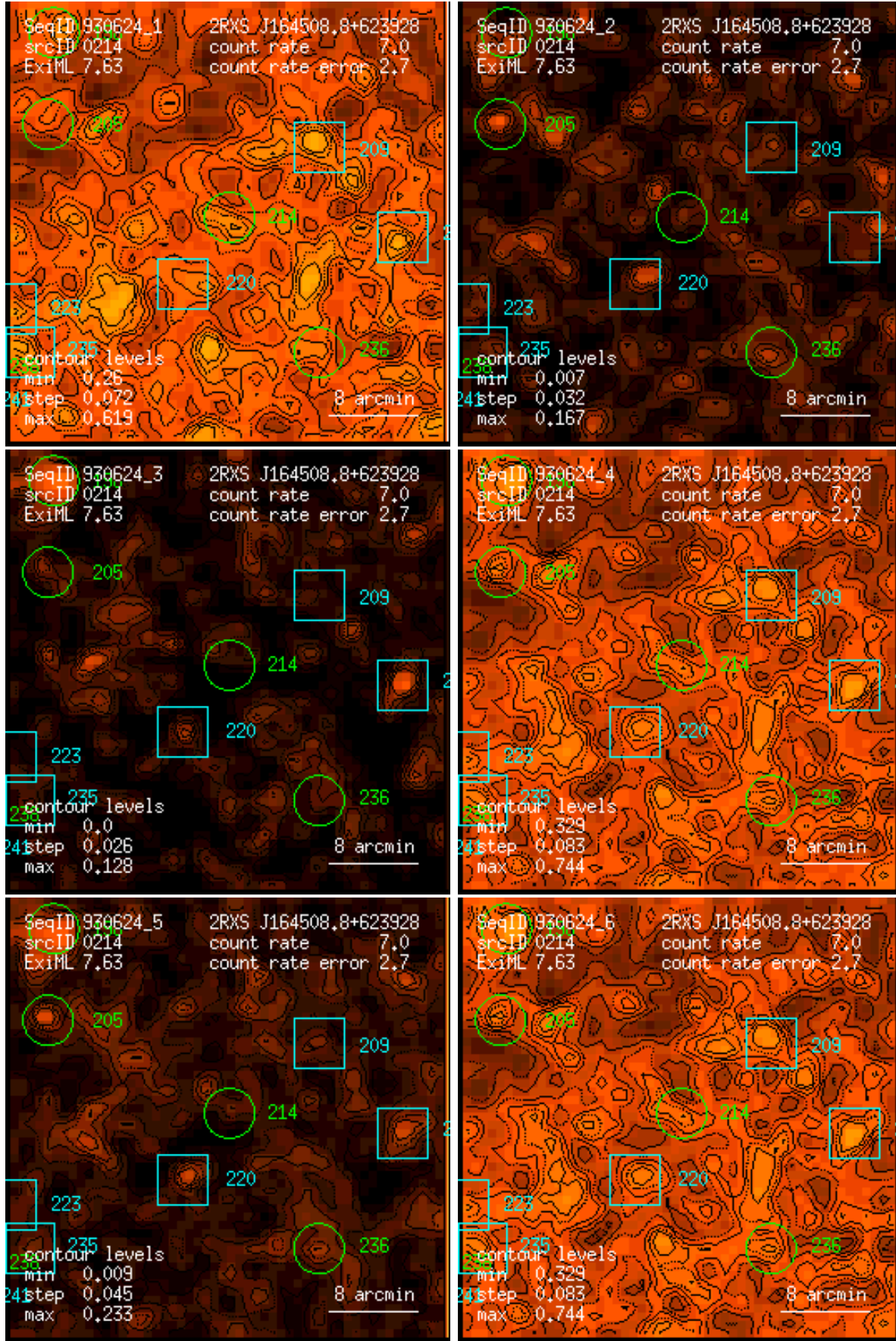
Figure 214: RASS 930624: detection 0214: band rate images, Gaussian filter: (1) PSPC channels 11 – 41, (2) 52 – 90, (3) 91 – 201, (4) 11 – 235, (5) 52 – 201, (6) 11 – 201. Broad band rates in counts/ks. Band rate contour levels in counts/ks/arcmin 2 .
