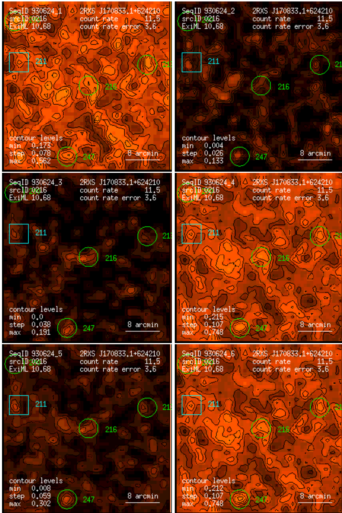
Figure 216: RASS 930624: detection 0216: band rate images, Gaussian filter: (1) PSPC channels 11 – 41, (2) 52 – 90, (3) 91 – 201, (4) 11 – 235, (5) 52 – 201, (6) 11 – 201. Broad band rates in counts/ks. Band rate contour levels in counts/ks/arcmin 2 .
