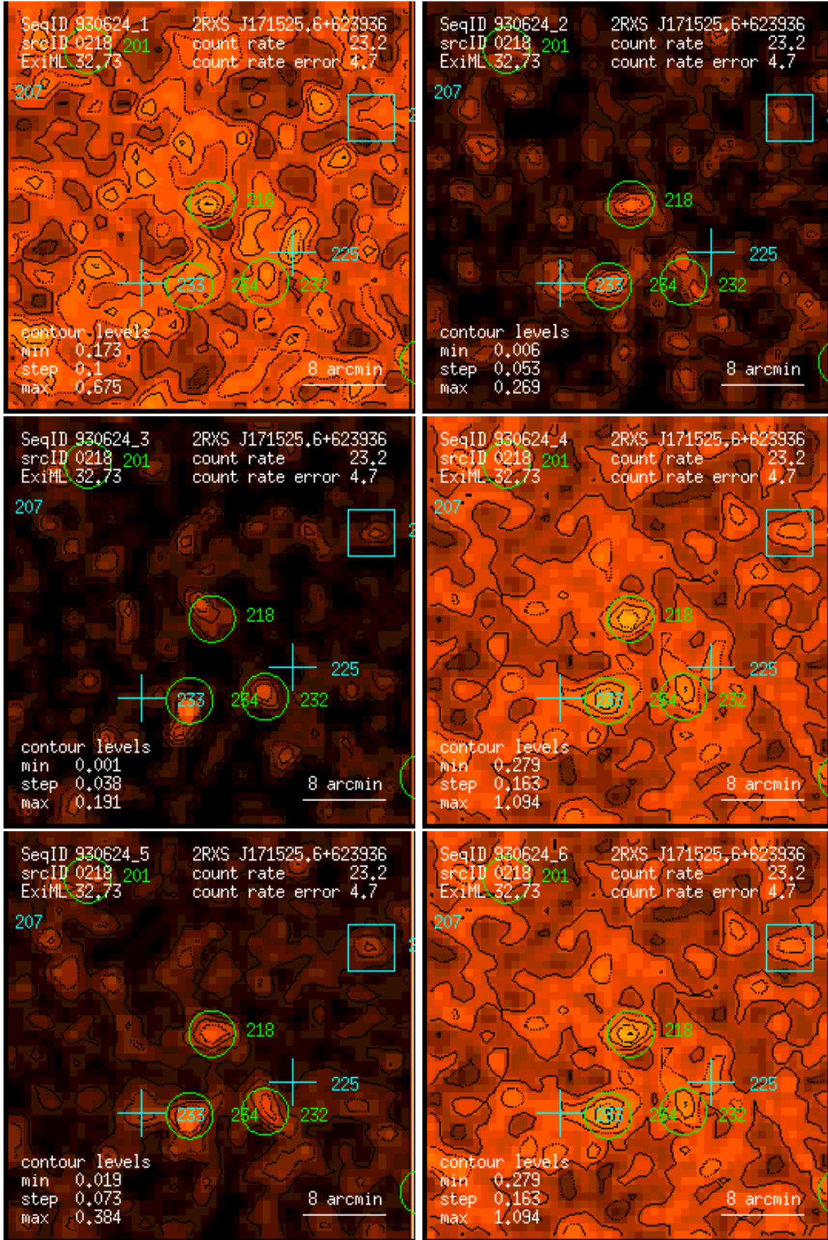
Figure 218: RASS 930624: detection 0218: band rate images, Gaussian filter: (1) PSPC channels 11 – 41, (2) 52 – 90, (3) 91 – 201, (4) 11 – 235, (5) 52 – 201, (6) 11 – 201. Broad band rates in counts/ks. Band rate contour levels in counts/ks/arcmin 2 .
