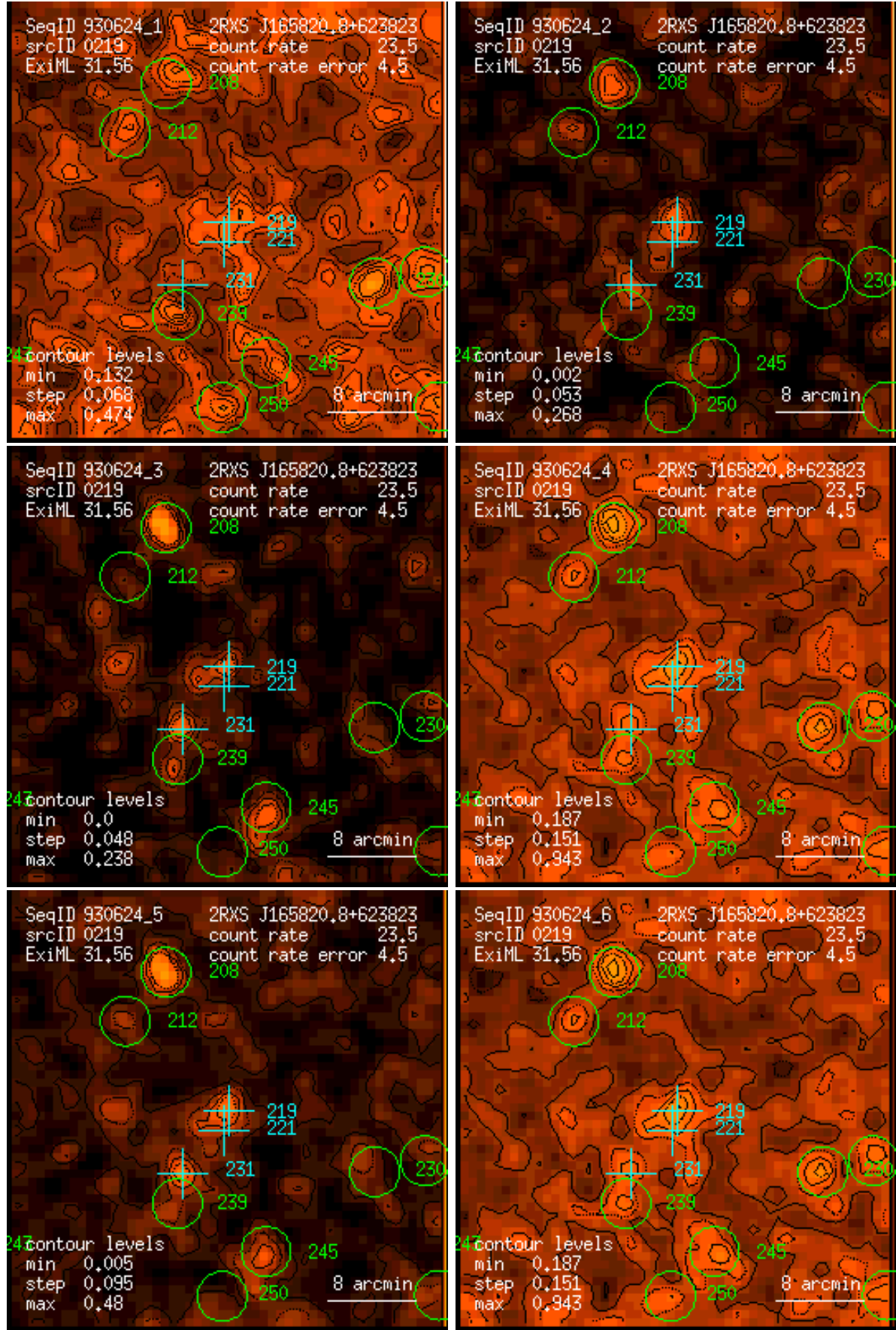
Figure 219: RASS 930624: detection 0219: band rate images, Gaussian filter: (1) PSPC channels 11 – 41, (2) 52 – 90, (3) 91 – 201, (4) 11 – 235, (5) 52 – 201, (6) 11 – 201. Broad band rates in counts/ks. Band rate contour levels in counts/ks/arcmin 2 .
