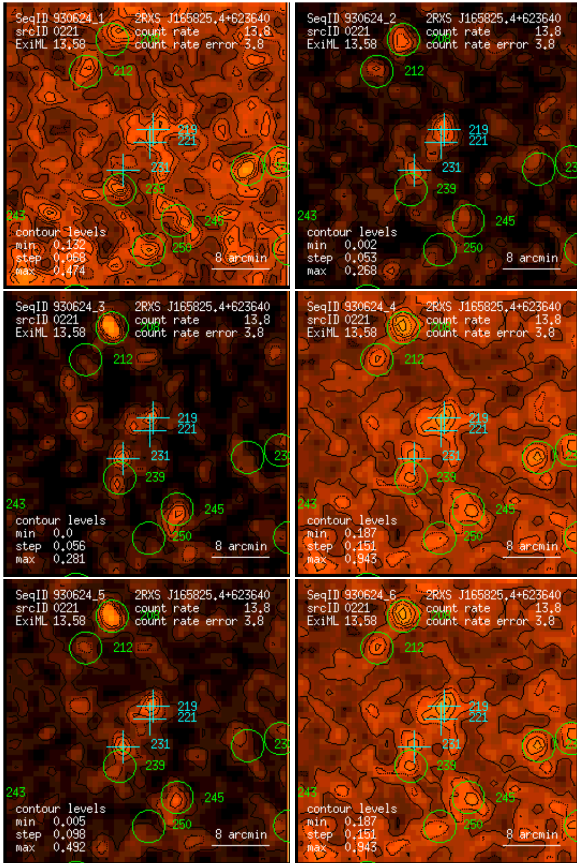
Figure 221: RASS 930624: detection 0221: band rate images, Gaussian filter: (1) PSPC channels 11 – 41, (2) 52 – 90, (3) 91 – 201, (4) 11 – 235, (5) 52 – 201, (6) 11 – 201. Broad band rates in counts/ks. Band rate contour levels in counts/ks/arcmin 2 .
