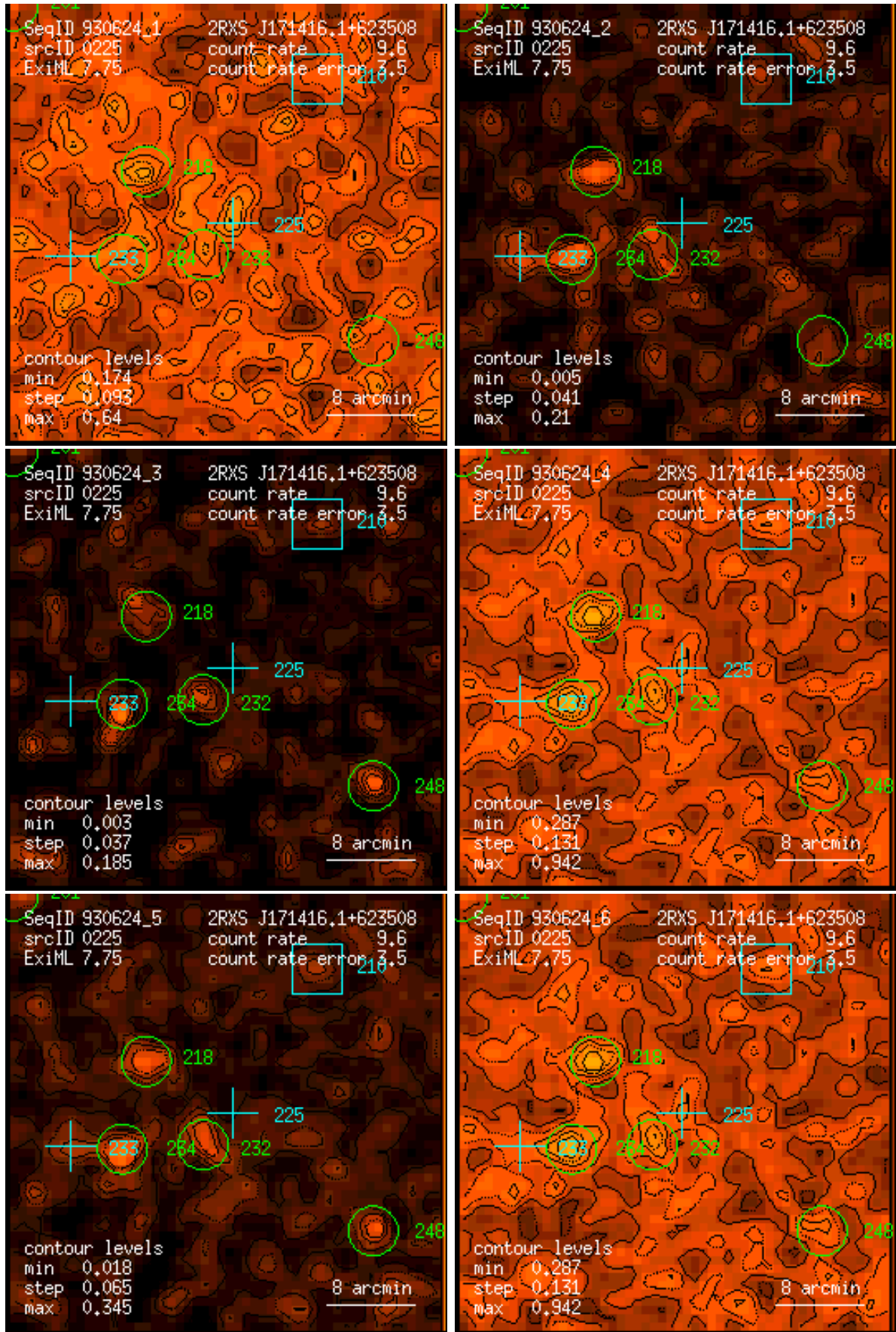
Figure 225: RASS 930624: detection 0225: band rate images, Gaussian filter: (1) PSPC channels 11 – 41, (2) 52 – 90, (3) 91 – 201, (4) 11 – 235, (5) 52 – 201, (6) 11 – 201. Broad band rates in counts/ks. Band rate contour levels in counts/ks/arcmin 2 .
