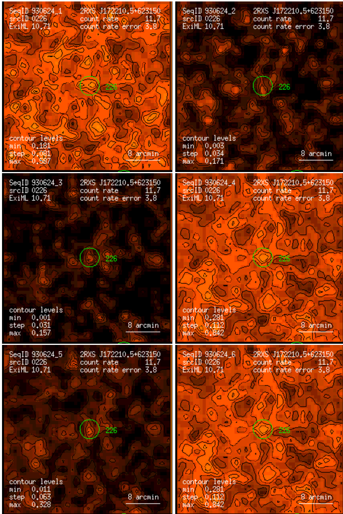
Figure 226: RASS 930624: detection 0226: band rate images, Gaussian filter: (1) PSPC channels 11 – 41, (2) 52 – 90, (3) 91 – 201, (4) 11 – 235, (5) 52 – 201, (6) 11 – 201. Broad band rates in counts/ks. Band rate contour levels in counts/ks/arcmin 2 .
