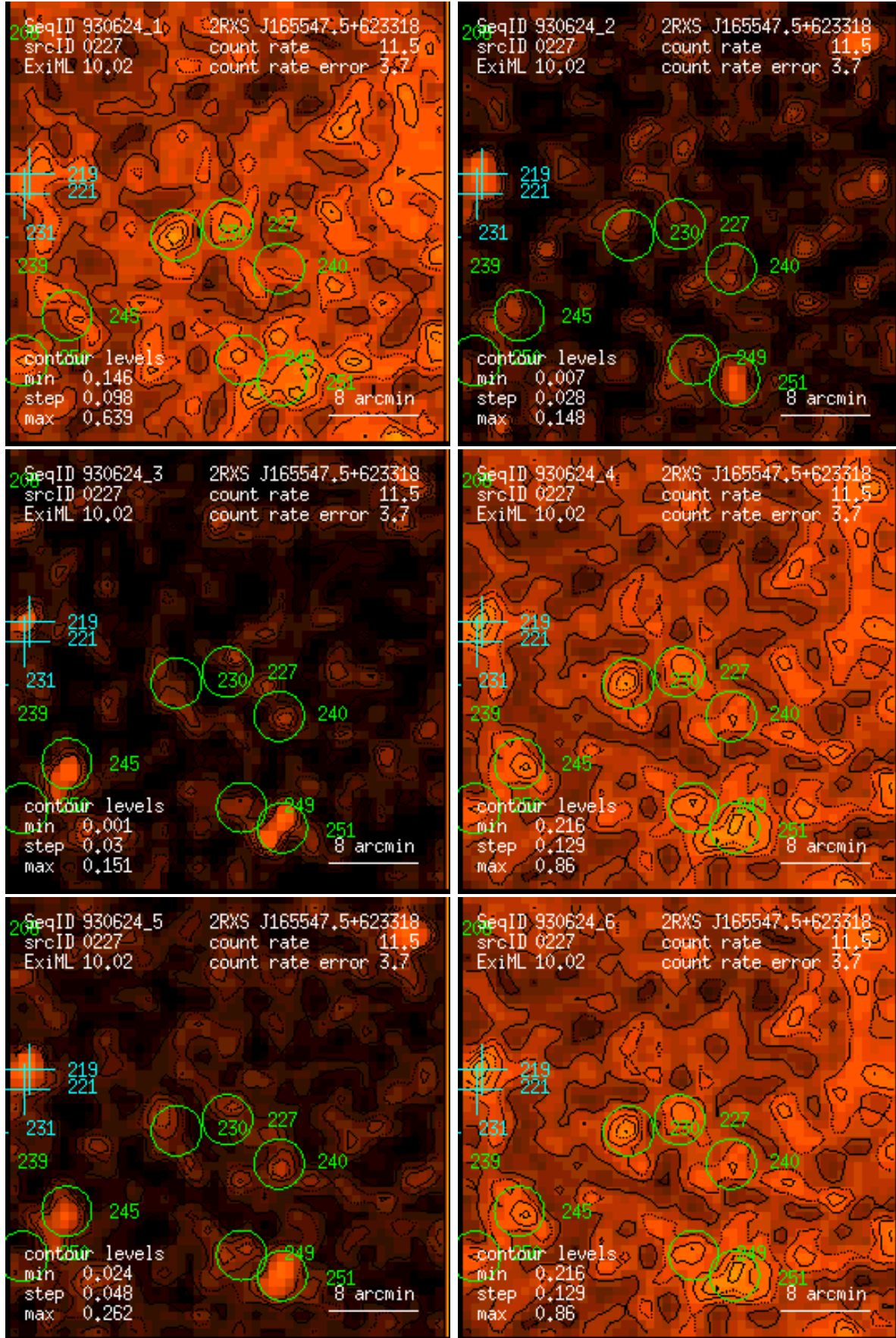
Figure 227: RASS 930624: detection 0227: band rate images, Gaussian filter: (1) PSPC channels 11 – 41, (2) 52 – 90, (3) 91 – 201, (4) 11 – 235, (5) 52 – 201, (6) 11 – 201. Broad band rates in counts/ks. Band rate contour levels in counts/ks/arcmin 2 .
