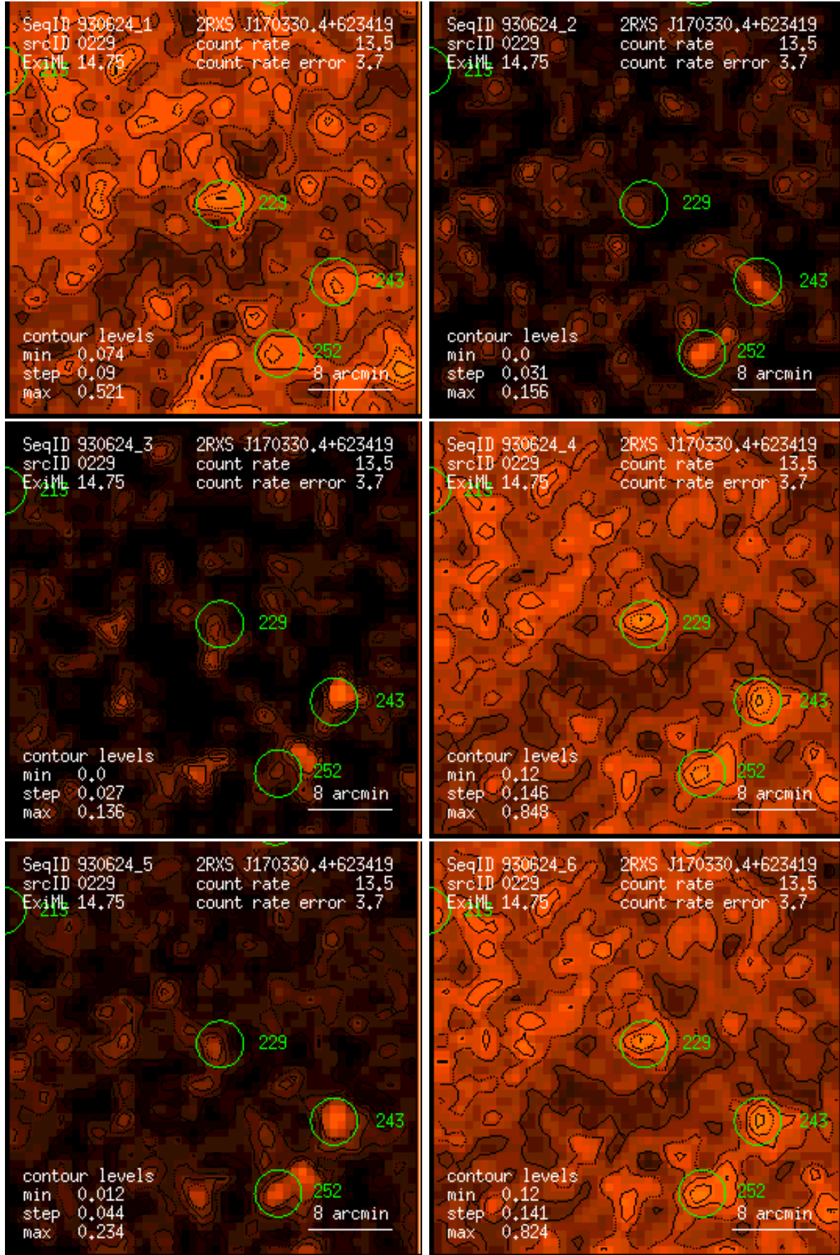
Figure 229: RASS 930624: detection 0229: band rate images, Gaussian filter: (1) PSPC channels 11 – 41, (2) 52 – 90, (3) 91 – 201, (4) 11 – 235, (5) 52 – 201, (6) 11 – 201. Broad band rates in counts/ks. Band rate contour levels in counts/ks/arcmin 2 .
