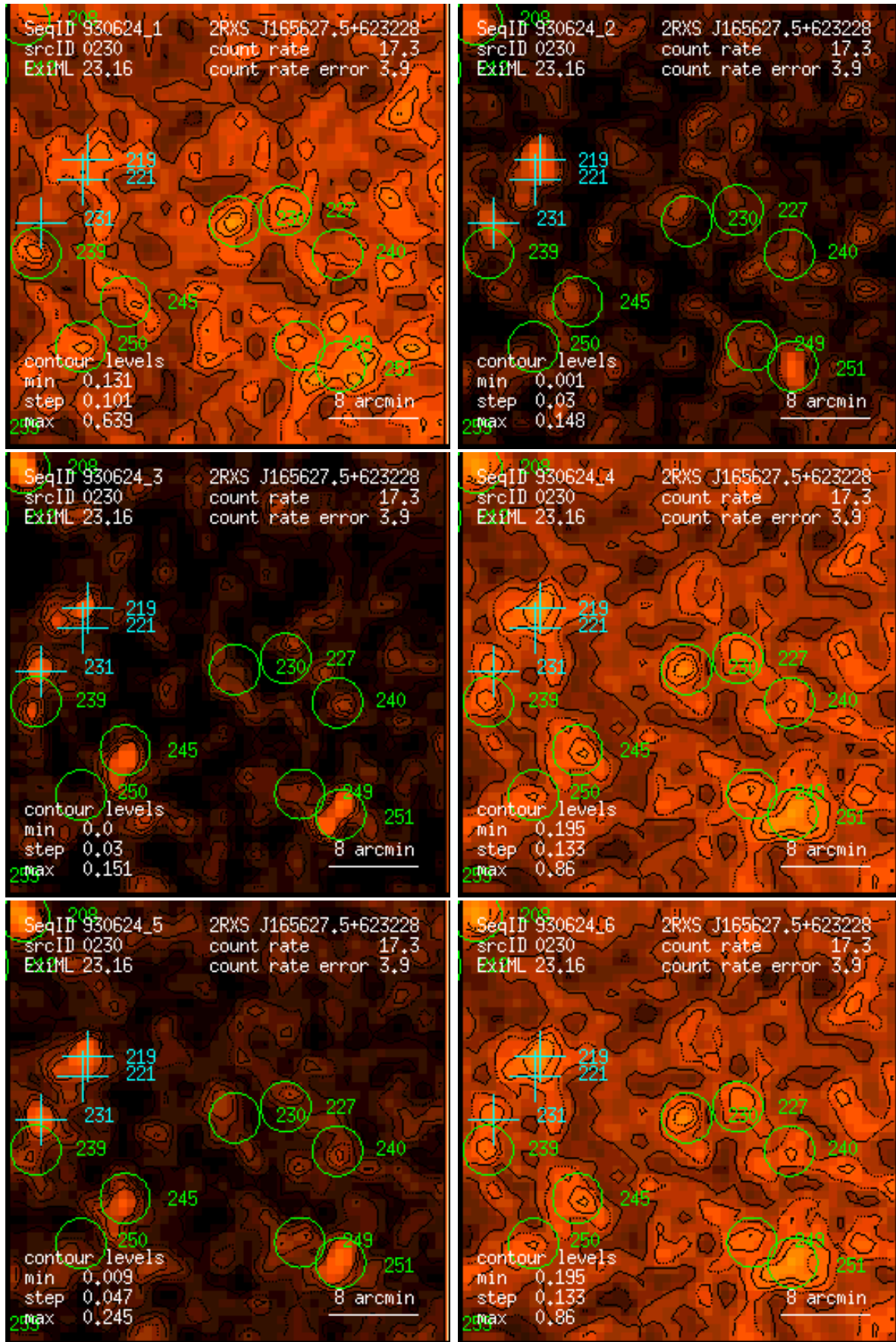
Figure 230: RASS 930624: detection 0230: band rate images, Gaussian filter: (1) PSPC channels 11 – 41, (2) 52 – 90, (3) 91 – 201, (4) 11 – 235, (5) 52 – 201, (6) 11 – 201. Broad band rates in counts/ks. Band rate contour levels in counts/ks/arcmin 2 .
