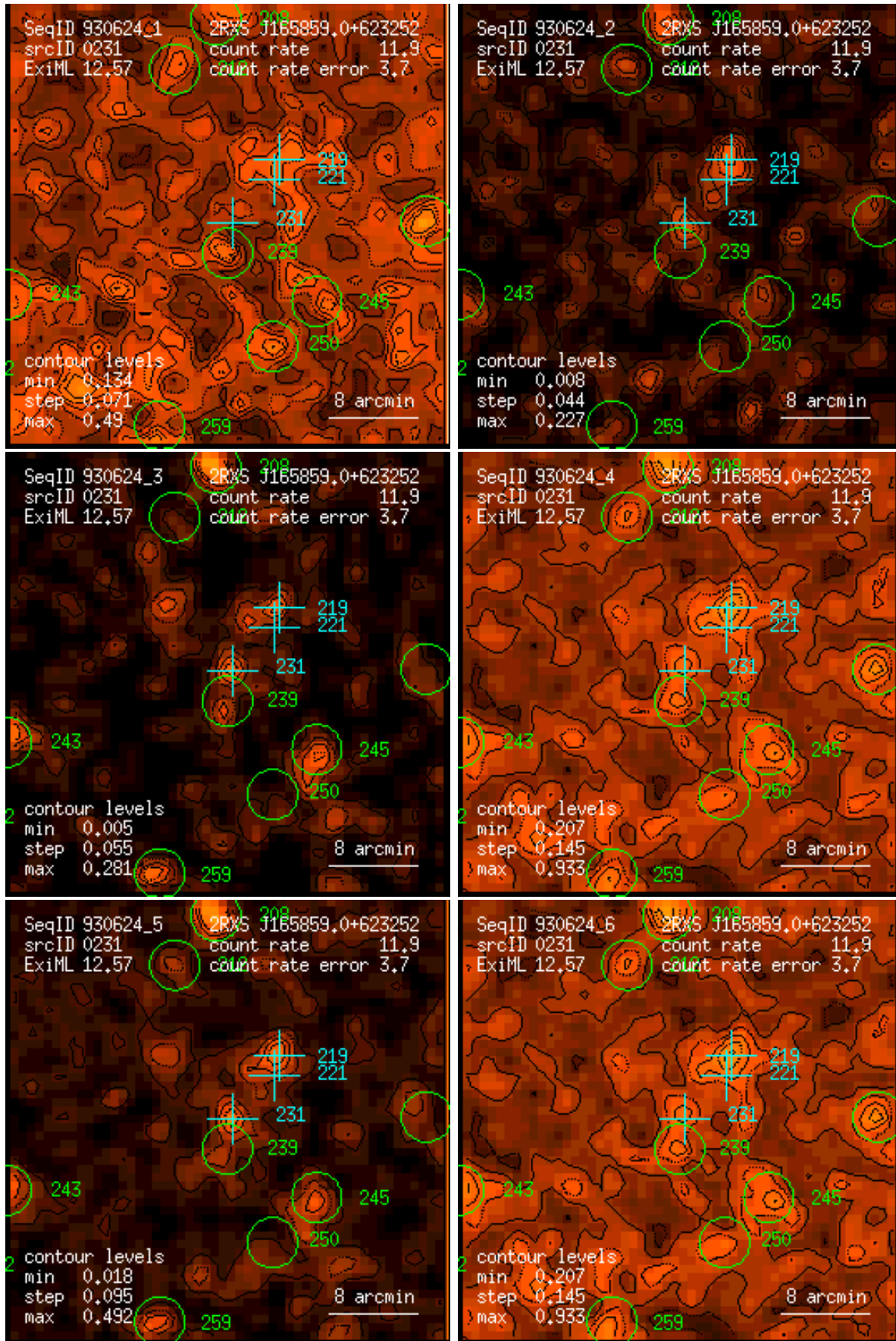
Figure 231: RASS 930624: detection 0231: band rate images, Gaussian filter: (1) PSPC channels 11 – 41, (2) 52 – 90, (3) 91 – 201, (4) 11 – 235, (5) 52 – 201, (6) 11 – 201. Broad band rates in counts/ks. Band rate contour levels in counts/ks/arcmin 2 .
