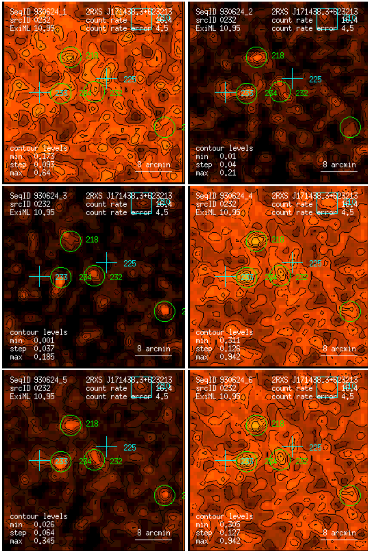
Figure 232: RASS 930624: detection 0232: band rate images, Gaussian filter: (1) PSPC channels 11 – 41, (2) 52 – 90, (3) 91 – 201, (4) 11 – 235, (5) 52 – 201, (6) 11 – 201. Broad band rates in counts/ks. Band rate contour levels in counts/ks/arcmin 2 .
