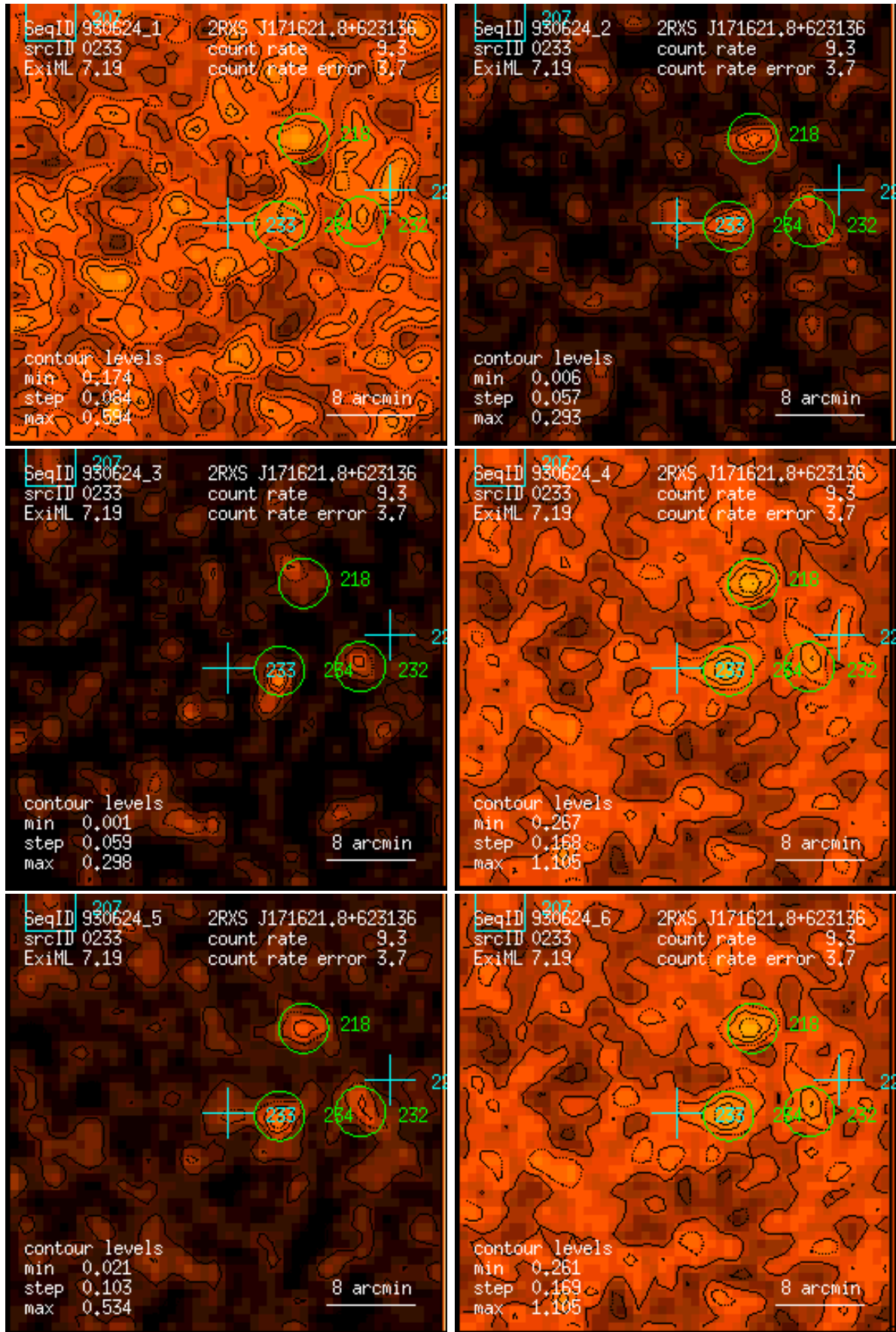
Figure 233: RASS 930624: detection 0233: band rate images, Gaussian filter: (1) PSPC channels 11 – 41, (2) 52 – 90, (3) 91 – 201, (4) 11 – 235, (5) 52 – 201, (6) 11 – 201. Broad band rates in counts/ks. Band rate contour levels in counts/ks/arcmin 2 .
