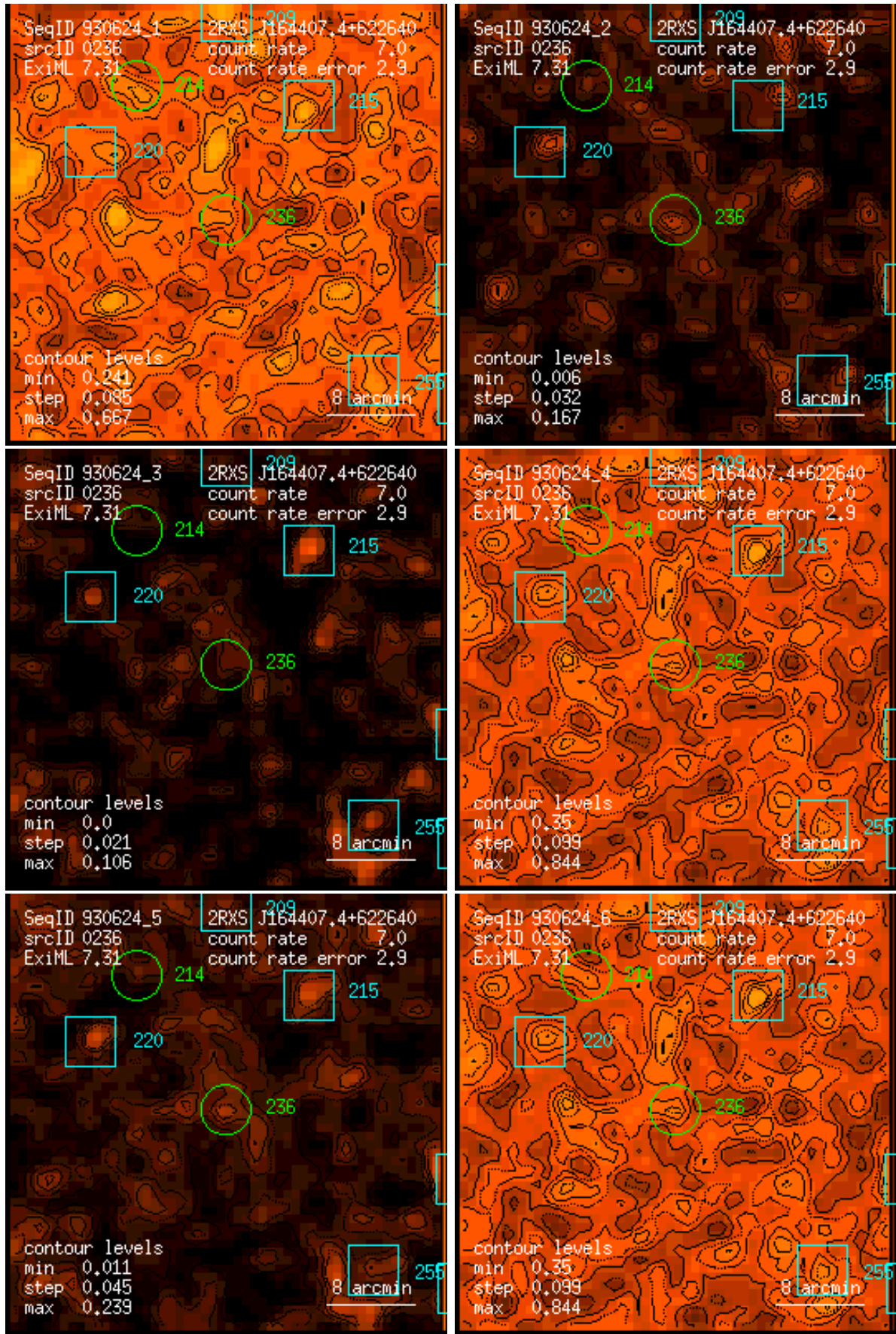
Figure 236: RASS 930624: detection 0236: band rate images, Gaussian filter: (1) PSPC channels 11 – 41, (2) 52 – 90, (3) 91 – 201, (4) 11 – 235, (5) 52 – 201, (6) 11 – 201. Broad band rates in counts/ks. Band rate contour levels in counts/ks/arcmin 2 .
