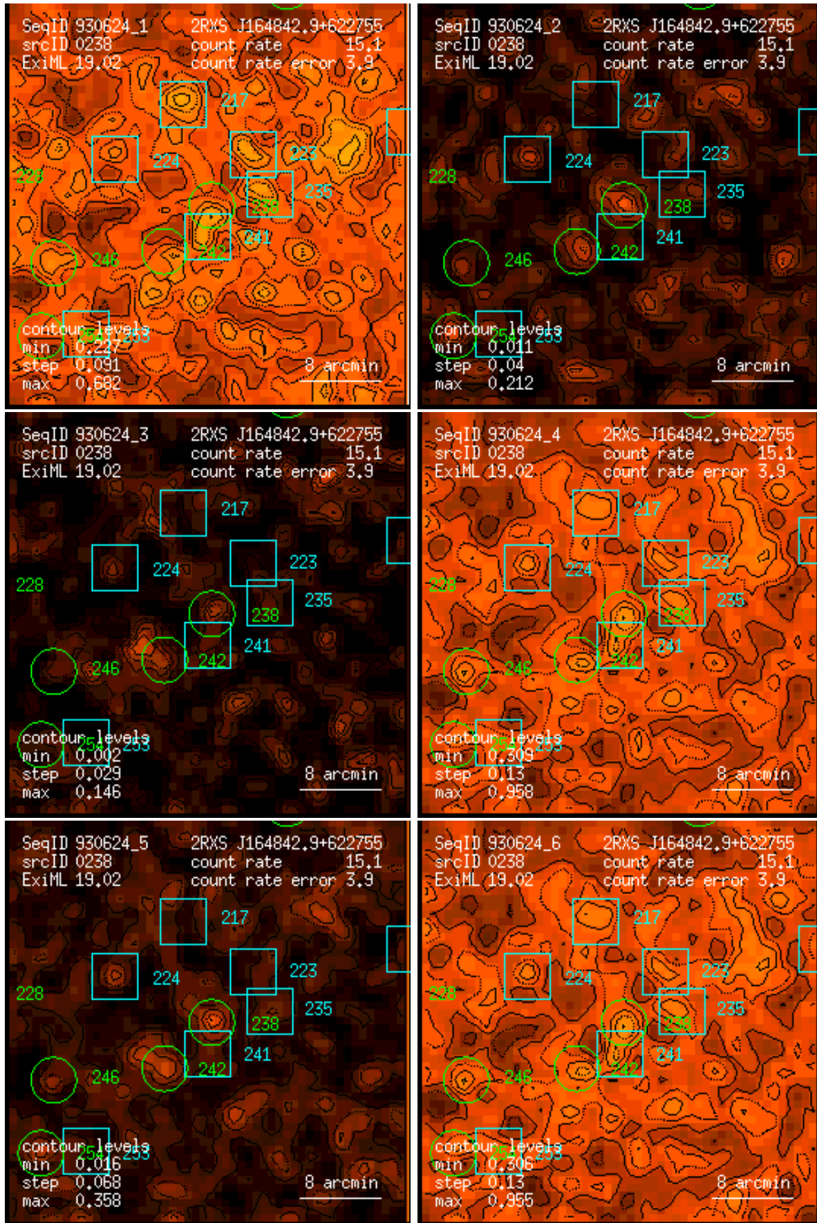
Figure 238: RASS 930624: detection 0238: band rate images, Gaussian filter: (1) PSPC channels 11 – 41, (2) 52 – 90, (3) 91 – 201, (4) 11 – 235, (5) 52 – 201, (6) 11 – 201. Broad band rates in counts/ks. Band rate contour levels in counts/ks/arcmin 2 .
