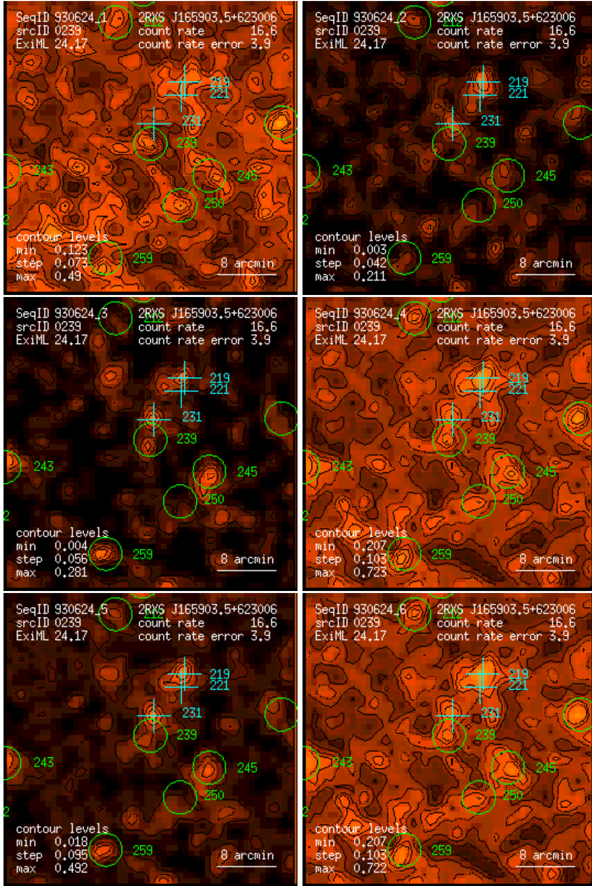
Figure 239: RASS 930624: detection 0239: band rate images, Gaussian filter: (1) PSPC channels 11 – 41, (2) 52 – 90, (3) 91 – 201, (4) 11 – 235, (5) 52 – 201, (6) 11 – 201. Broad band rates in counts/ks. Band rate contour levels in counts/ks/arcmin 2 .
