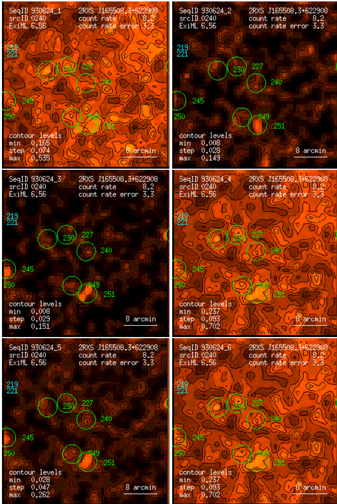
Figure 240: RASS 930624: detection 0240: band rate images, Gaussian filter: (1) PSPC channels 11 – 41, (2) 52 – 90, (3) 91 – 201, (4) 11 – 235, (5) 52 – 201, (6) 11 – 201. Broad band rates in counts/ks. Band rate contour levels in counts/ks/arcmin 2 .
