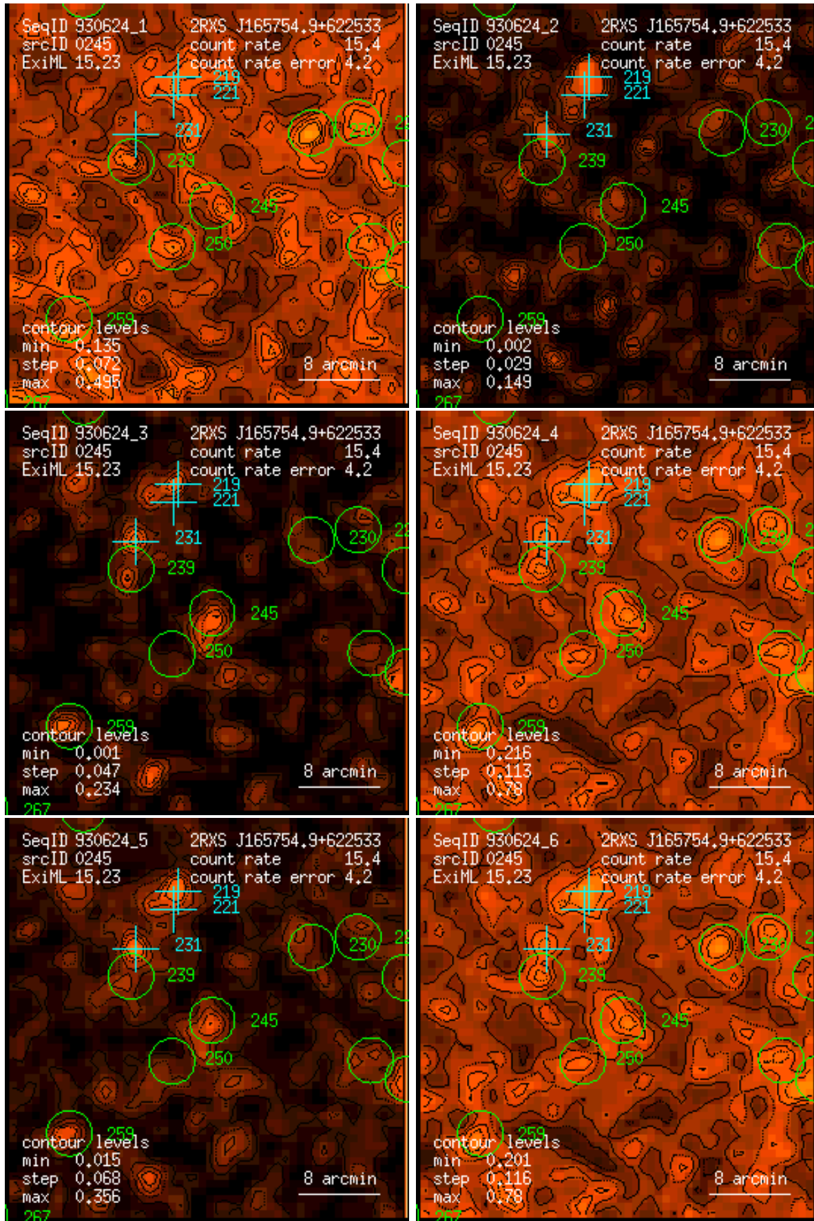
Figure 245: RASS 930624: detection 0245: band rate images, Gaussian filter: (1) PSPC channels 11 – 41, (2) 52 – 90, (3) 91 – 201, (4) 11 – 235, (5) 52 – 201, (6) 11 – 201. Broad band rates in counts/ks. Band rate contour levels in counts/ks/arcmin 2 .
