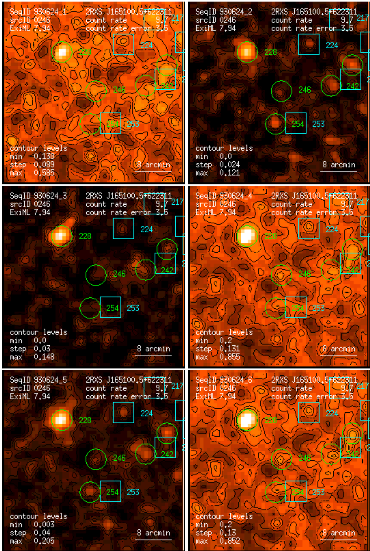
Figure 246: RASS 930624: detection 0246: band rate images, Gaussian filter: (1) PSPC channels 11 – 41, (2) 52 – 90, (3) 91 – 201, (4) 11 – 235, (5) 52 – 201, (6) 11 – 201. Broad band rates in counts/ks. Band rate contour levels in counts/ks/arcmin 2 .
