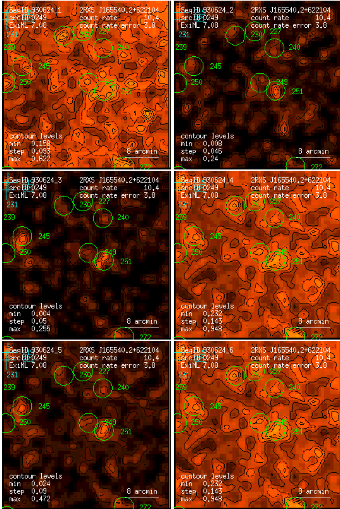
Figure 249: RASS 930624: detection 0249: band rate images, Gaussian filter: (1) PSPC channels 11 – 41, (2) 52 – 90, (3) 91 – 201, (4) 11 – 235, (5) 52 – 201, (6) 11 – 201. Broad band rates in counts/ks. Band rate contour levels in counts/ks/arcmin 2 .
