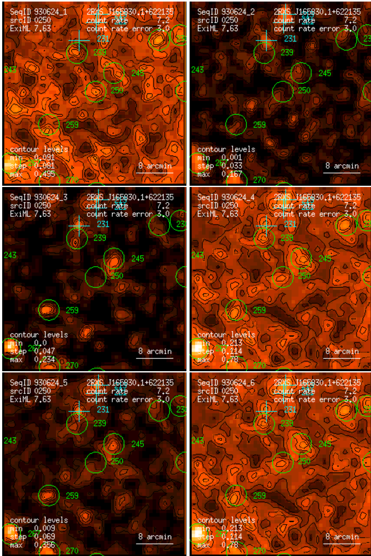
Figure 250: RASS 930624: detection 0250: band rate images, Gaussian filter: (1) PSPC channels 11 – 41, (2) 52 – 90, (3) 91 – 201, (4) 11 – 235, (5) 52 – 201, (6) 11 – 201. Broad band rates in counts/ks. Band rate contour levels in counts/ks/arcmin 2 .
