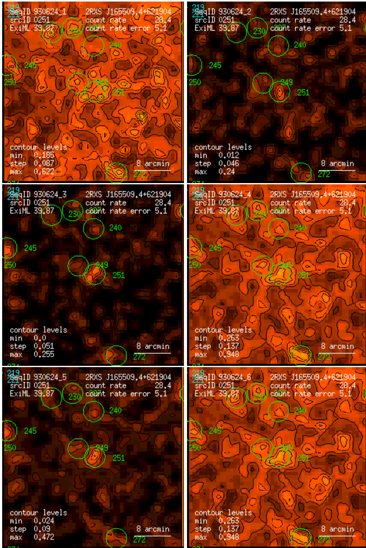
Figure 251: RASS 930624: detection 0251: band rate images, Gaussian filter: (1) PSPC channels 11 – 41, (2) 52 – 90, (3) 91 – 201, (4) 11 – 235, (5) 52 – 201, (6) 11 – 201. Broad band rates in counts/ks. Band rate contour levels in counts/ks/arcmin 2 .
