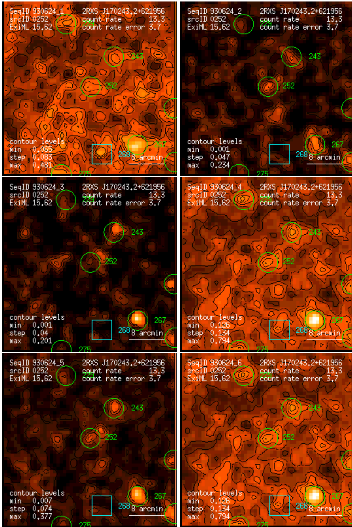
Figure 252: RASS 930624: detection 0252: band rate images, Gaussian filter: (1) PSPC channels 11 – 41, (2) 52 – 90, (3) 91 – 201, (4) 11 – 235, (5) 52 – 201, (6) 11 – 201. Broad band rates in counts/ks. Band rate contour levels in counts/ks/arcmin 2 .
