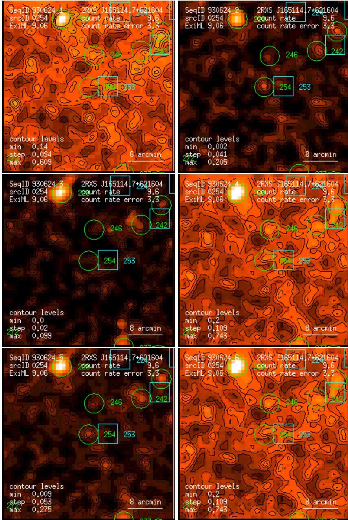
Figure 254: RASS 930624: detection 0254: band rate images, Gaussian filter: (1) PSPC channels 11 – 41, (2) 52 – 90, (3) 91 – 201, (4) 11 – 235, (5) 52 – 201, (6) 11 – 201. Broad band rates in counts/ks. Band rate contour levels in counts/ks/arcmin 2 .
