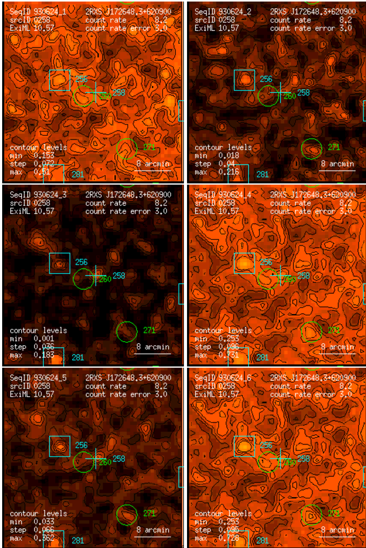
Figure 258: RASS 930624: detection 0258: band rate images, Gaussian filter: (1) PSPC channels 11 – 41, (2) 52 – 90, (3) 91 – 201, (4) 11 – 235, (5) 52 – 201, (6) 11 – 201. Broad band rates in counts/ks. Band rate contour levels in counts/ks/arcmin 2 .
