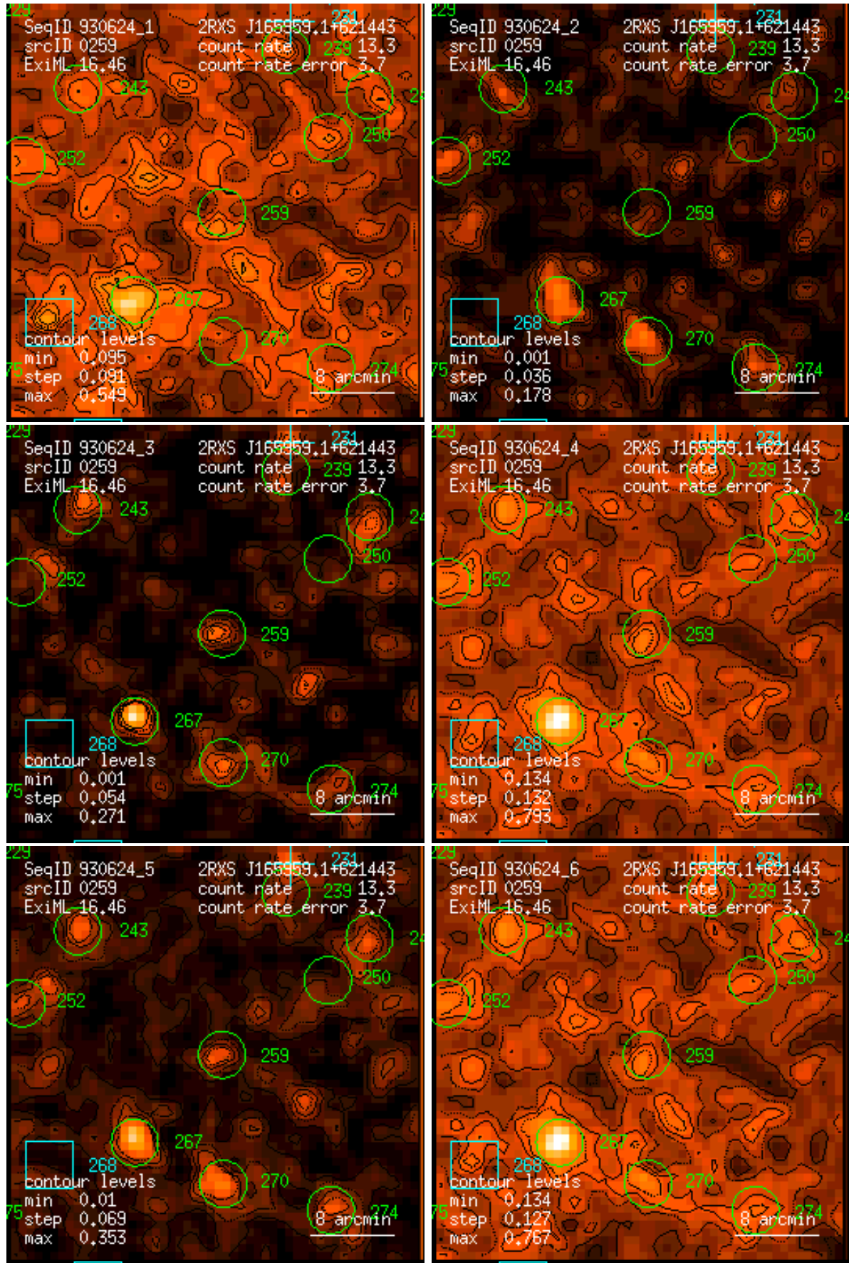
Figure 259: RASS 930624: detection 0259: band rate images, Gaussian filter: (1) PSPC channels 11 – 41, (2) 52 – 90, (3) 91 – 201, (4) 11 – 235, (5) 52 – 201, (6) 11 – 201. Broad band rates in counts/ks. Band rate contour levels in counts/ks/arcmin 2 .
