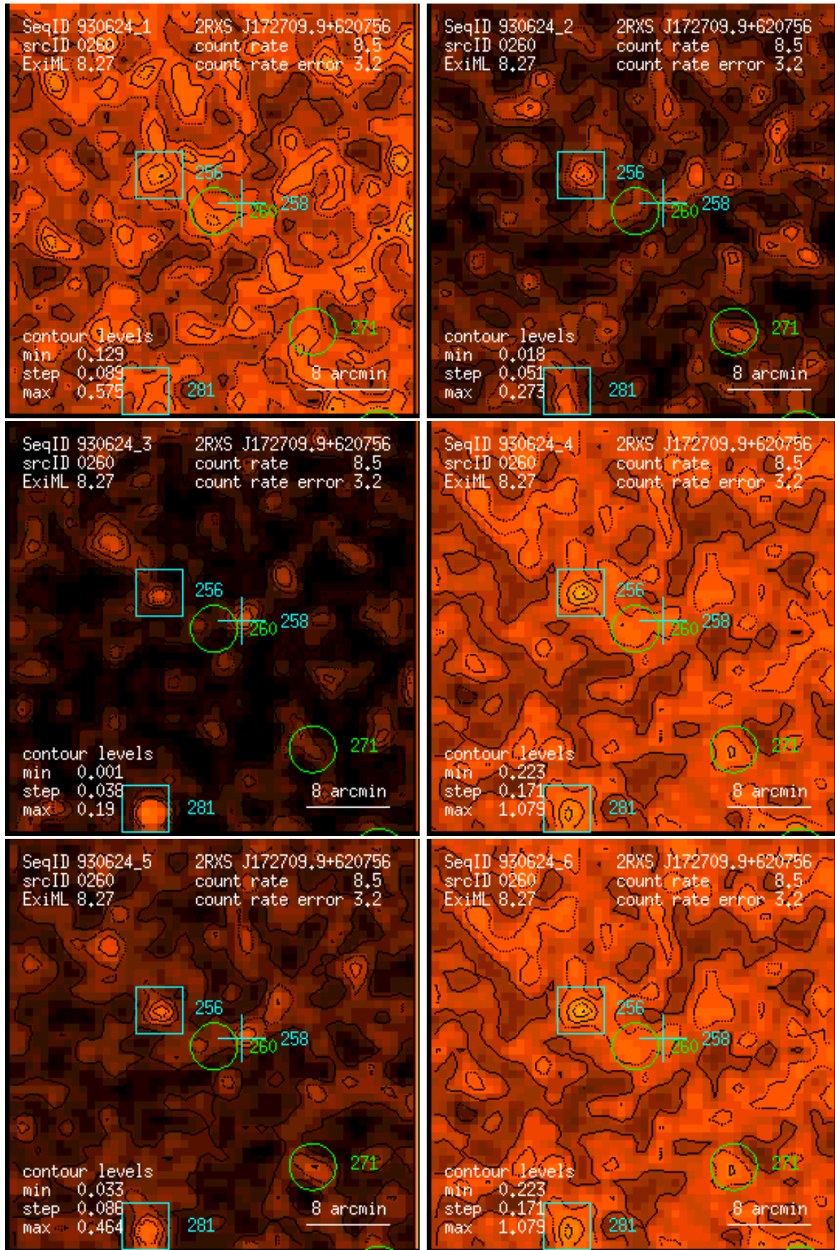
Figure 260: RASS 930624: detection 0260: band rate images, Gaussian filter: (1) PSPC channels 11 – 41, (2) 52 – 90, (3) 91 – 201, (4) 11 – 235, (5) 52 – 201, (6) 11 – 201. Broad band rates in counts/ks. Band rate contour levels in counts/ks/arcmin 2 .
