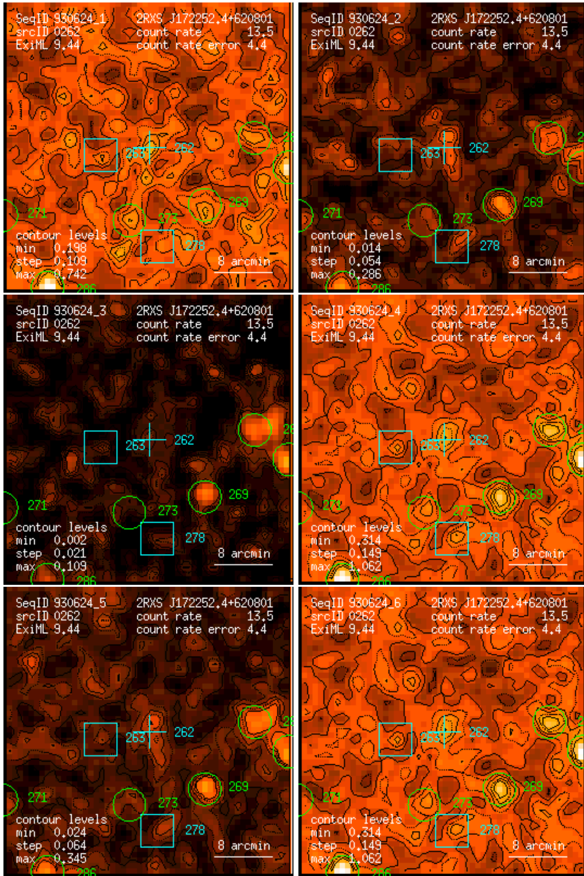
Figure 262: RASS 930624: detection 0262: band rate images, Gaussian filter: (1) PSPC channels 11 – 41, (2) 52 – 90, (3) 91 – 201, (4) 11 – 235, (5) 52 – 201, (6) 11 – 201. Broad band rates in counts/ks. Band rate contour levels in counts/ks/arcmin 2 .
