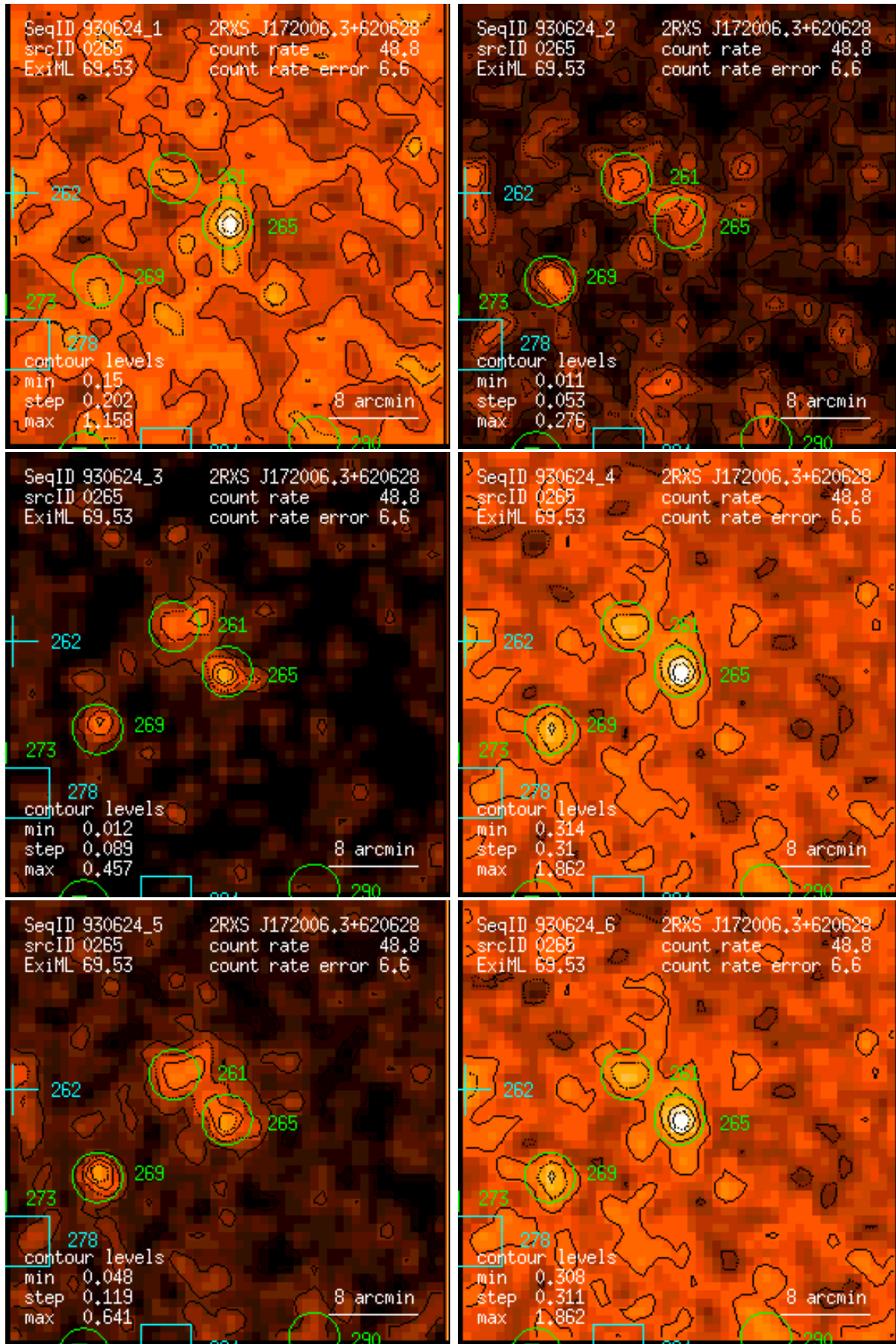
Figure 265: RASS 930624: detection 0265: band rate images, Gaussian filter: (1) PSPC channels 11 – 41, (2) 52 – 90, (3) 91 – 201, (4) 11 – 235, (5) 52 – 201, (6) 11 – 201. Broad band rates in counts/ks. Band rate contour levels in counts/ks/arcmin 2 .
