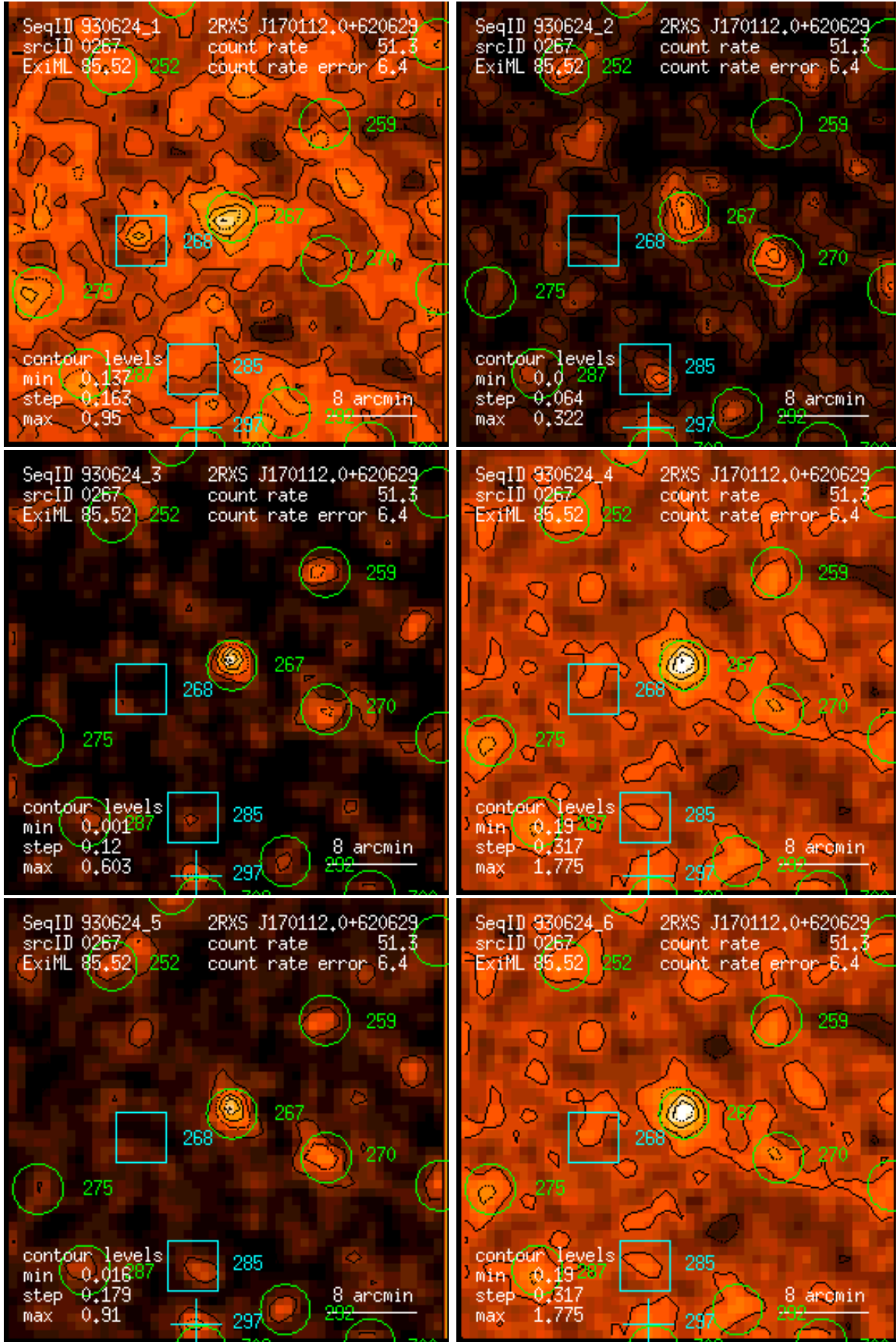
Figure 267: RASS 930624: detection 0267: band rate images, Gaussian filter: (1) PSPC channels 11 – 41, (2) 52 – 90, (3) 91 – 201, (4) 11 – 235, (5) 52 – 201, (6) 11 – 201. Broad band rates in counts/ks. Band rate contour levels in counts/ks/arcmin 2 .
