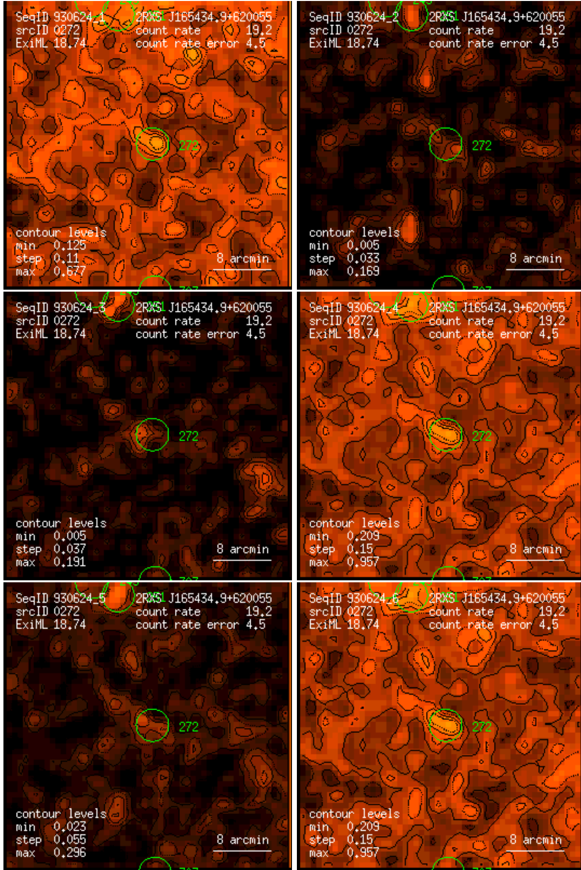
Figure 272: RASS 930624: detection 0272: band rate images, Gaussian filter: (1) PSPC channels 11 – 41, (2) 52 – 90, (3) 91 – 201, (4) 11 – 235, (5) 52 – 201, (6) 11 – 201. Broad band rates in counts/ks. Band rate contour levels in counts/ks/arcmin 2 .
