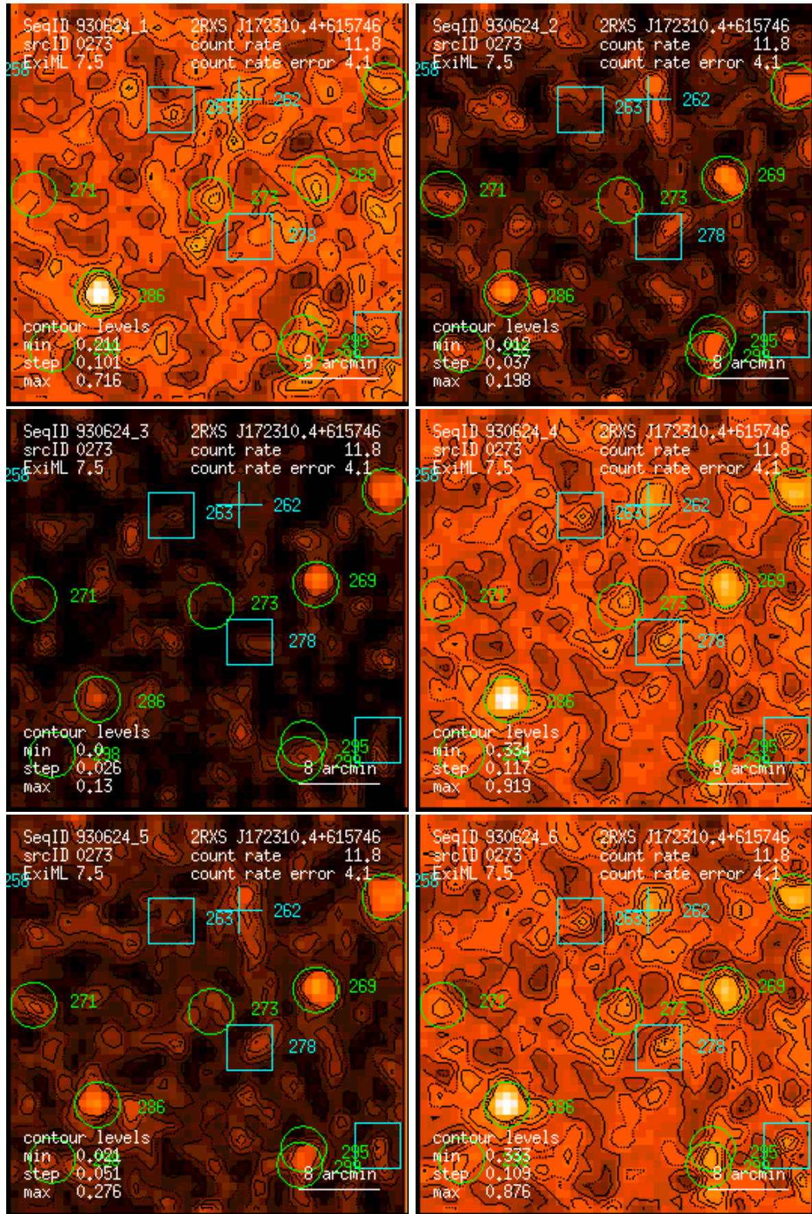
Figure 273: RASS 930624: detection 0273: band rate images, Gaussian filter: (1) PSPC channels 11 – 41, (2) 52 – 90, (3) 91 – 201, (4) 11 – 235, (5) 52 – 201, (6) 11 – 201. Broad band rates in counts/ks. Band rate contour levels in counts/ks/arcmin 2 .
