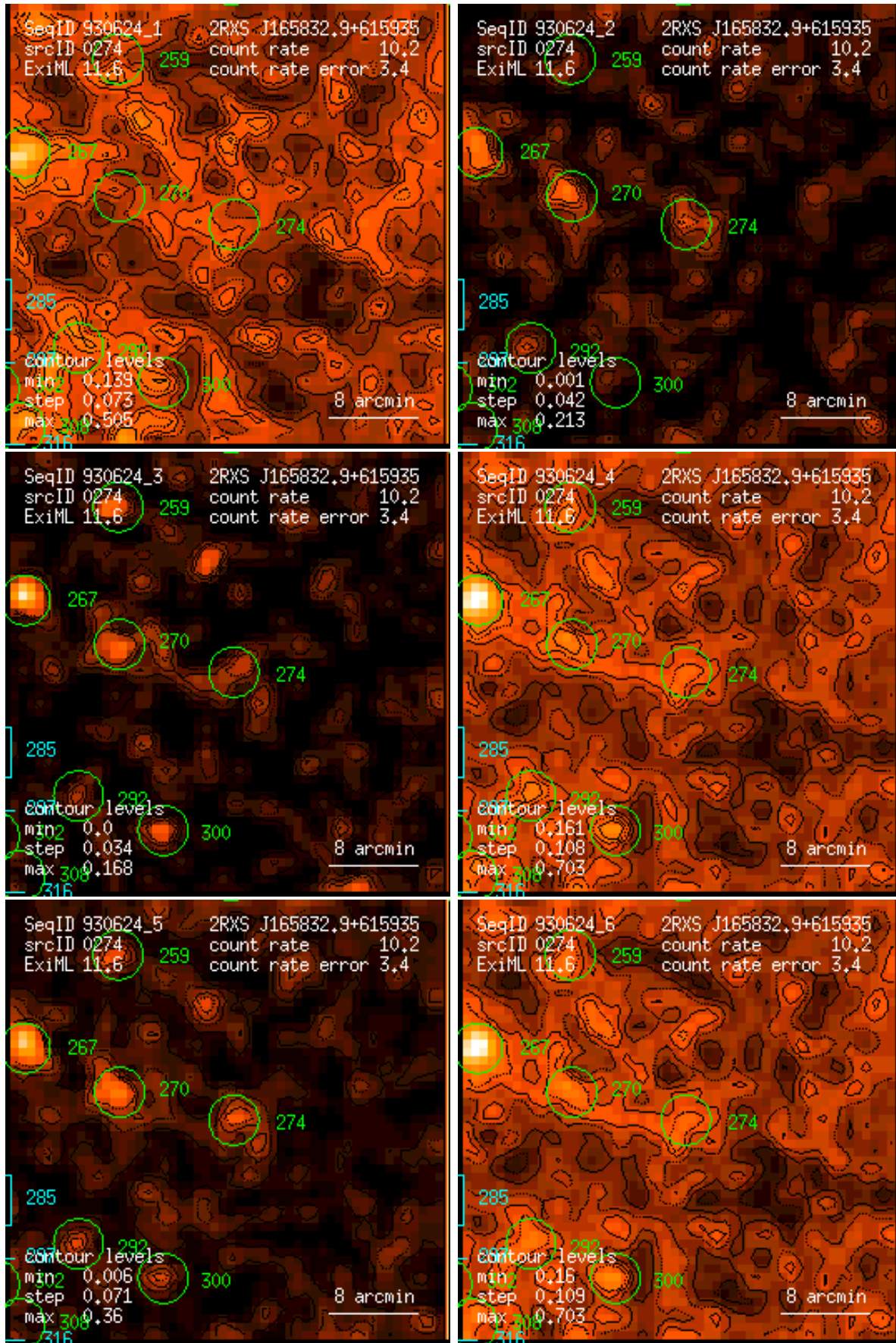
Figure 274: RASS 930624: detection 0274: band rate images, Gaussian filter: (1) PSPC channels 11 – 41, (2) 52 – 90, (3) 91 – 201, (4) 11 – 235, (5) 52 – 201, (6) 11 – 201. Broad band rates in counts/ks. Band rate contour levels in counts/ks/arcmin 2 .
