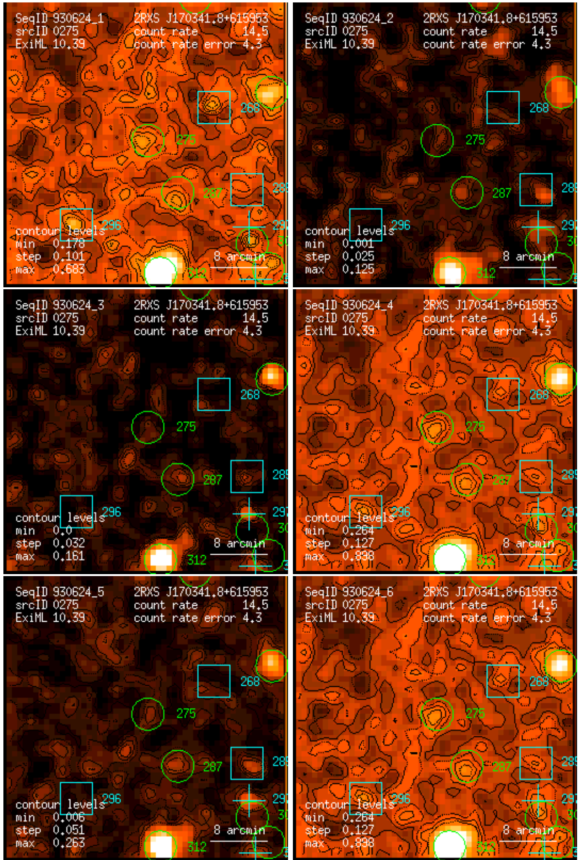
Figure 275: RASS 930624: detection 0275: band rate images, Gaussian filter: (1) PSPC channels 11 – 41, (2) 52 – 90, (3) 91 – 201, (4) 11 – 235, (5) 52 – 201, (6) 11 – 201. Broad band rates in counts/ks. Band rate contour levels in counts/ks/arcmin 2 .
