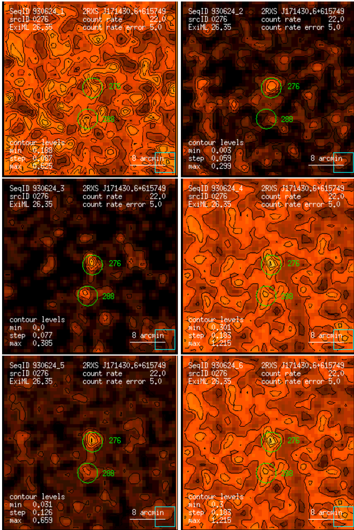
Figure 276: RASS 930624: detection 0276: band rate images, Gaussian filter: (1) PSPC channels 11 – 41, (2) 52 – 90, (3) 91 – 201, (4) 11 – 235, (5) 52 – 201, (6) 11 – 201. Broad band rates in counts/ks. Band rate contour levels in counts/ks/arcmin 2 .
