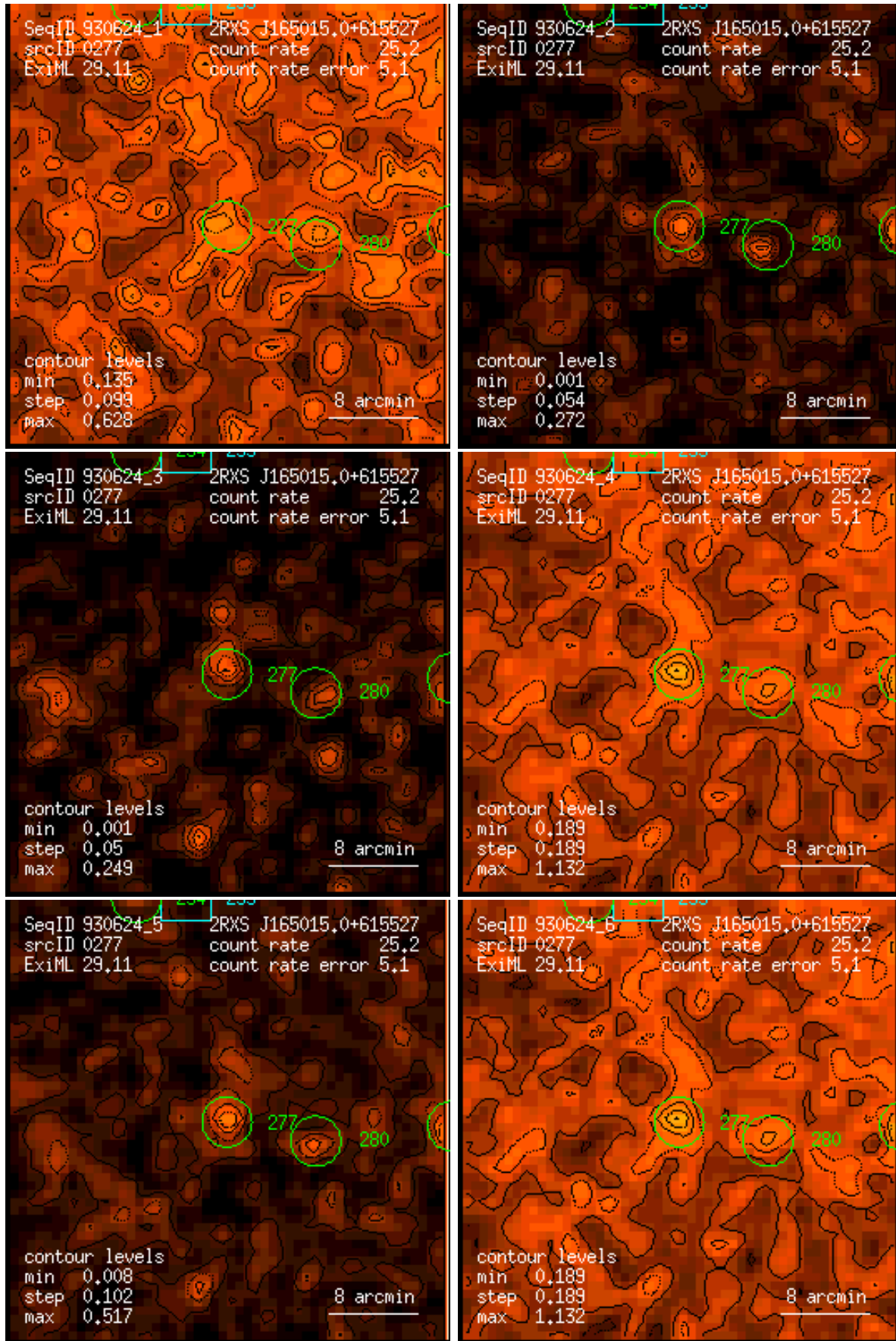
Figure 277: RASS 930624: detection 0277: band rate images, Gaussian filter: (1) PSPC channels 11 – 41, (2) 52 – 90, (3) 91 – 201, (4) 11 – 235, (5) 52 – 201, (6) 11 – 201. Broad band rates in counts/ks. Band rate contour levels in counts/ks/arcmin 2 .
