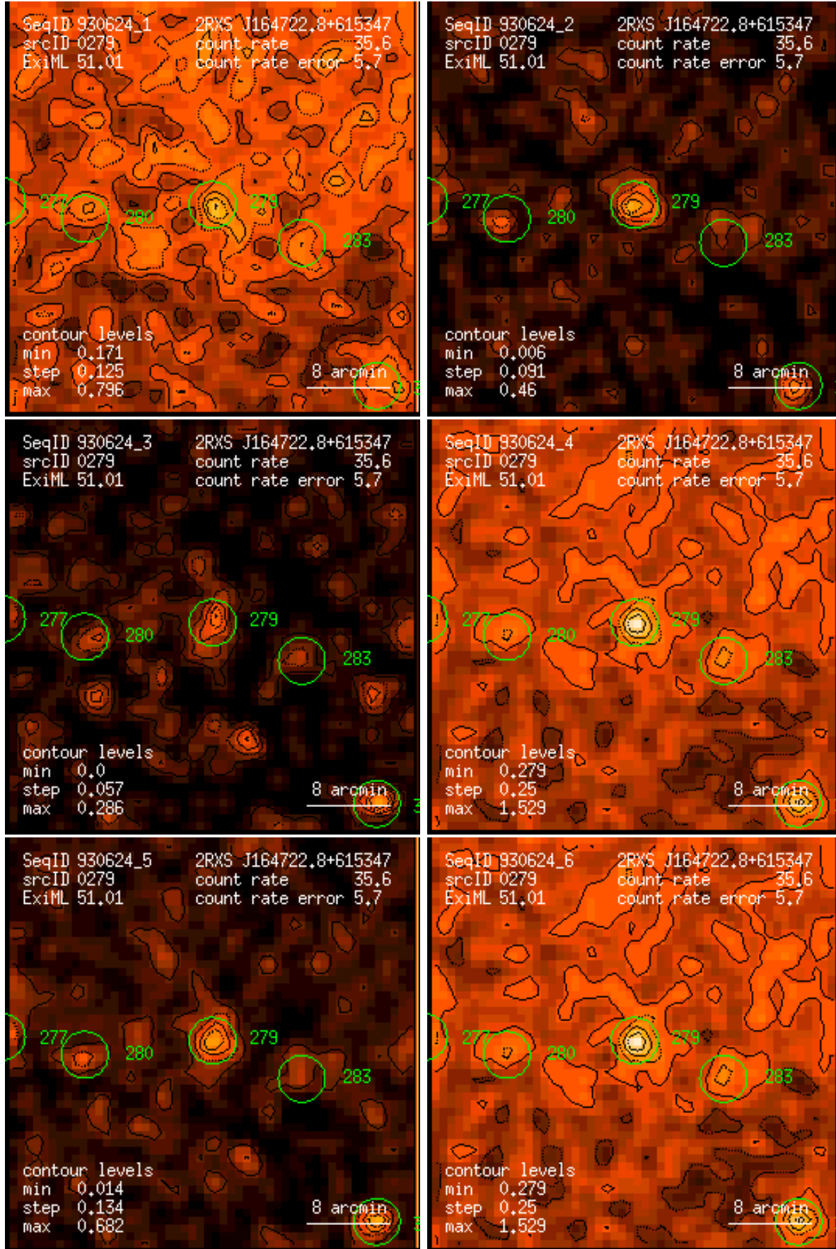
Figure 279: RASS 930624: detection 0279: band rate images, Gaussian filter: (1) PSPC channels 11 – 41, (2) 52 – 90, (3) 91 – 201, (4) 11 – 235, (5) 52 – 201, (6) 11 – 201. Broad band rates in counts/ks. Band rate contour levels in counts/ks/arcmin 2 .
