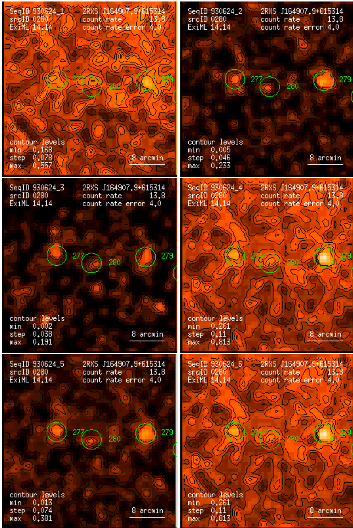
Figure 280: RASS 930624: detection 0280: band rate images, Gaussian filter: (1) PSPC channels 11 – 41, (2) 52 – 90, (3) 91 – 201, (4) 11 – 235, (5) 52 – 201, (6) 11 – 201. Broad band rates in counts/ks. Band rate contour levels in counts/ks/arcmin 2 .
