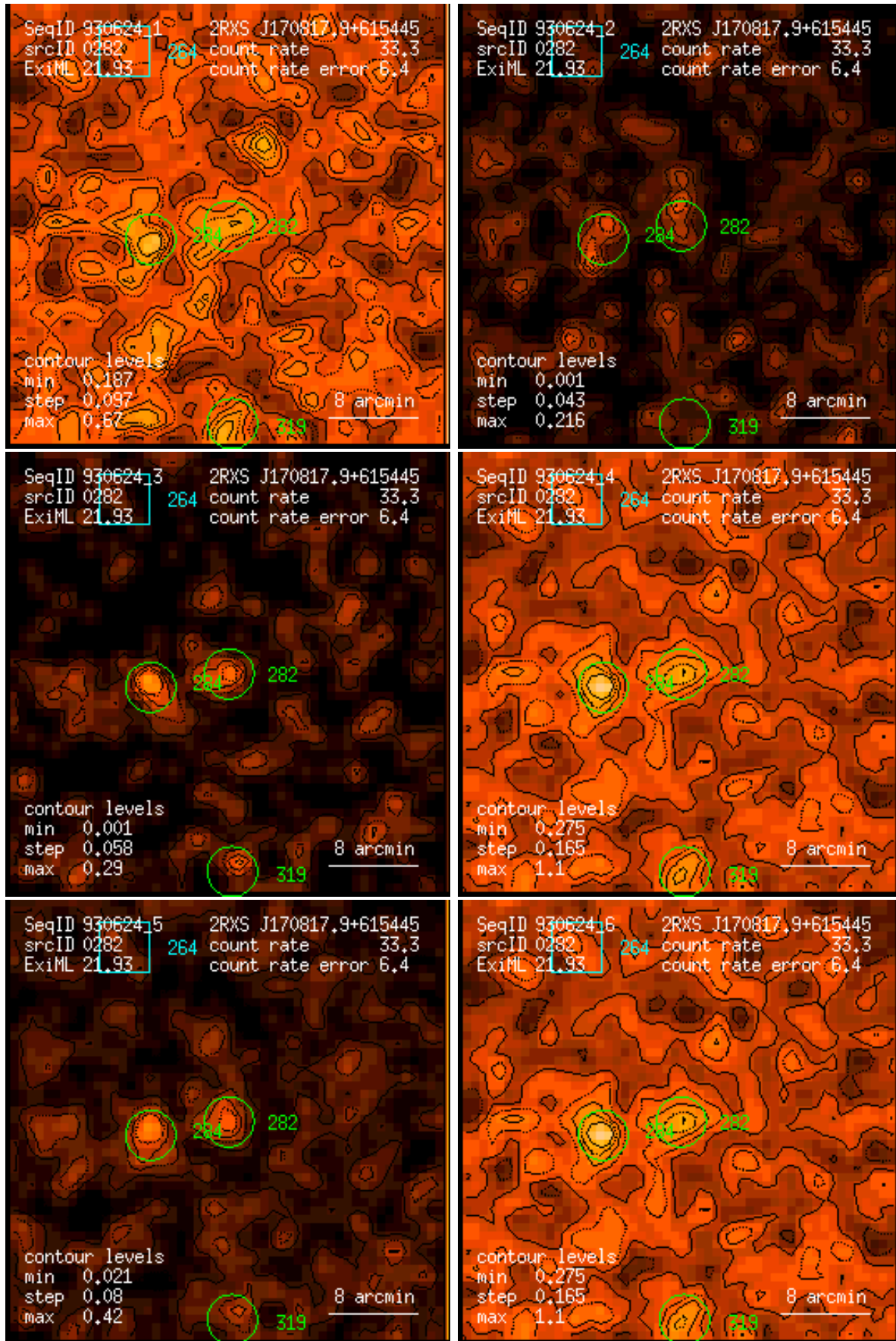
Figure 282: RASS 930624: detection 0282: band rate images, Gaussian filter: (1) PSPC channels 11 – 41, (2) 52 – 90, (3) 91 – 201, (4) 11 – 235, (5) 52 – 201, (6) 11 – 201. Broad band rates in counts/ks. Band rate contour levels in counts/ks/arcmin 2 .
