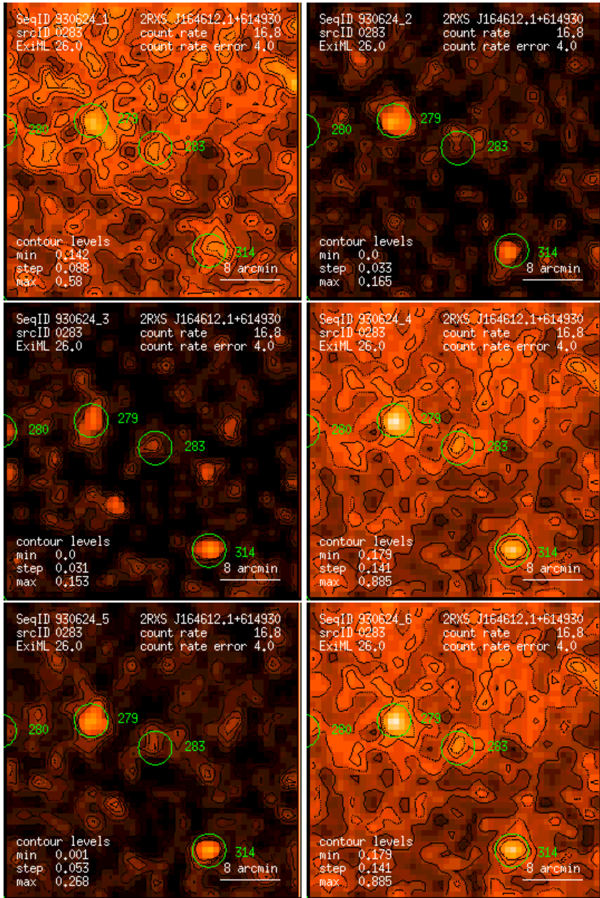
Figure 283: RASS 930624: detection 0283: band rate images, Gaussian filter: (1) PSPC channels 11 – 41, (2) 52 – 90, (3) 91 – 201, (4) 11 – 235, (5) 52 – 201, (6) 11 – 201. Broad band rates in counts/ks. Band rate contour levels in counts/ks/arcmin 2 .
