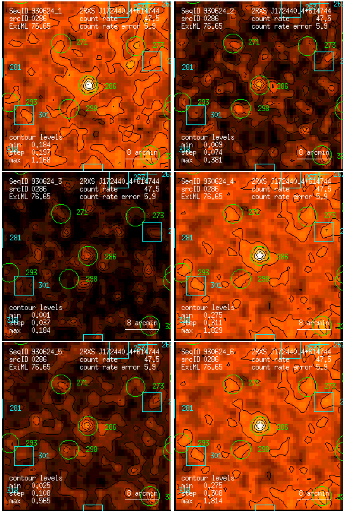
Figure 286: RASS 930624: detection 0286: band rate images, Gaussian filter: (1) PSPC channels 11 – 41, (2) 52 – 90, (3) 91 – 201, (4) 11 – 235, (5) 52 – 201, (6) 11 – 201. Broad band rates in counts/ks. Band rate contour levels in counts/ks/arcmin 2 .
