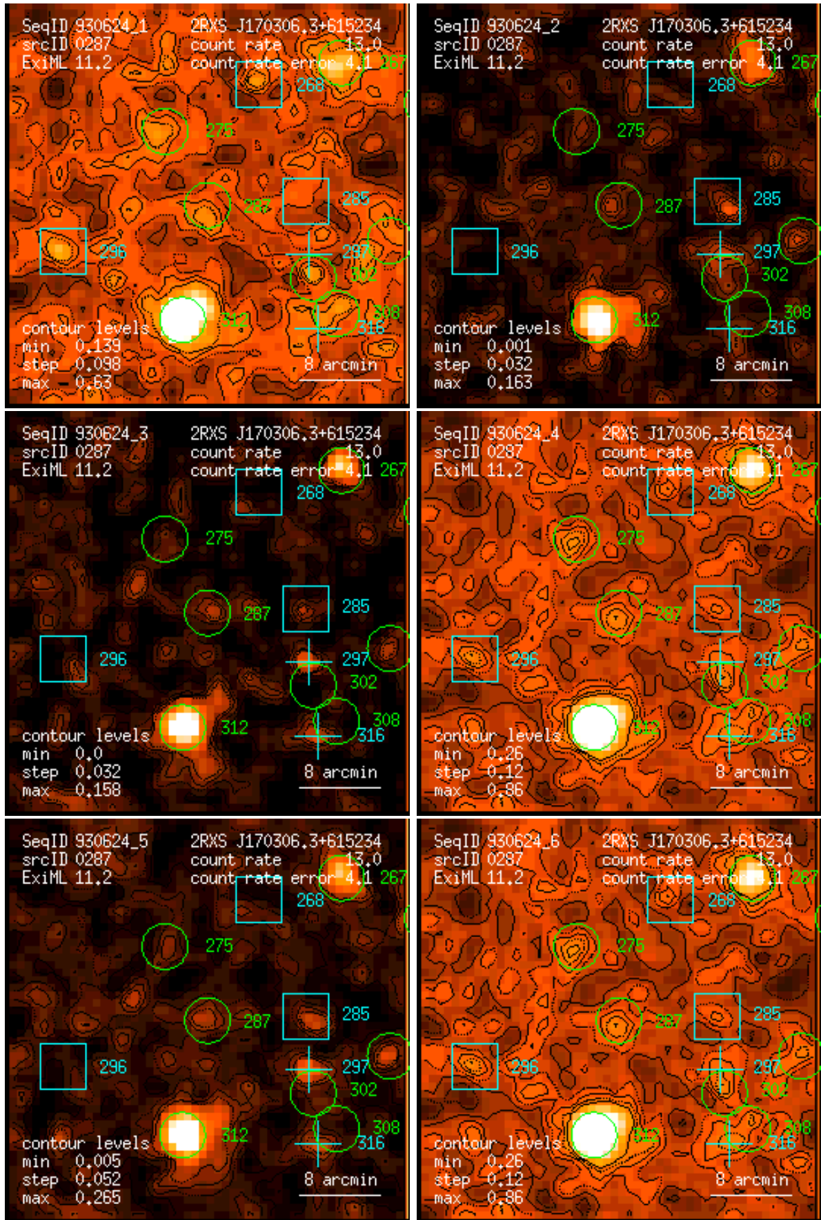
Figure 287: RASS 930624: detection 0287: band rate images, Gaussian filter: (1) PSPC channels 11 – 41, (2) 52 – 90, (3) 91 – 201, (4) 11 – 235, (5) 52 – 201, (6) 11 – 201. Broad band rates in counts/ks. Band rate contour levels in counts/ks/arcmin 2 .
