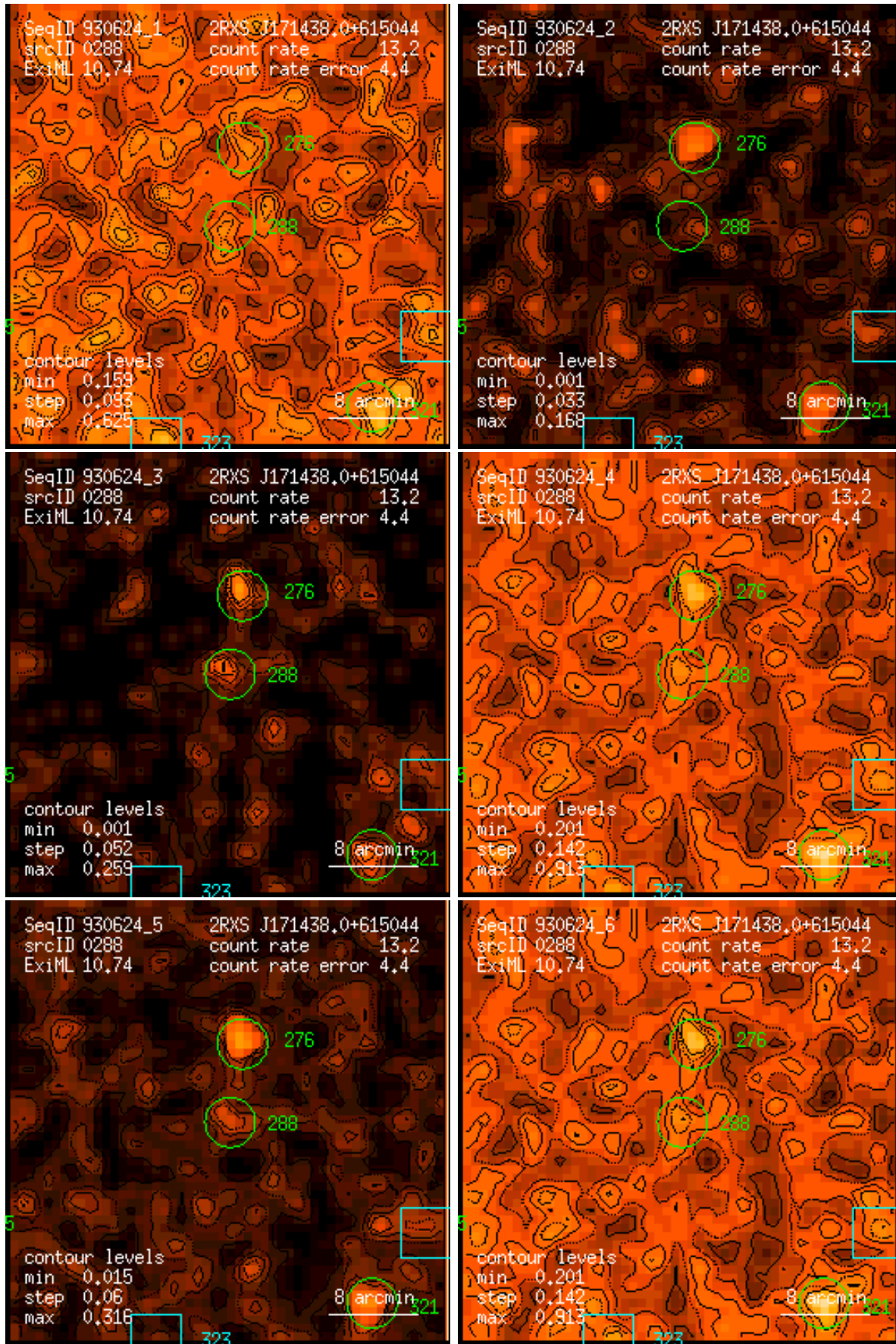
Figure 288: RASS 930624: detection 0288: band rate images, Gaussian filter: (1) PSPC channels 11 – 41, (2) 52 – 90, (3) 91 – 201, (4) 11 – 235, (5) 52 – 201, (6) 11 – 201. Broad band rates in counts/ks. Band rate contour levels in counts/ks/arcmin 2 .
