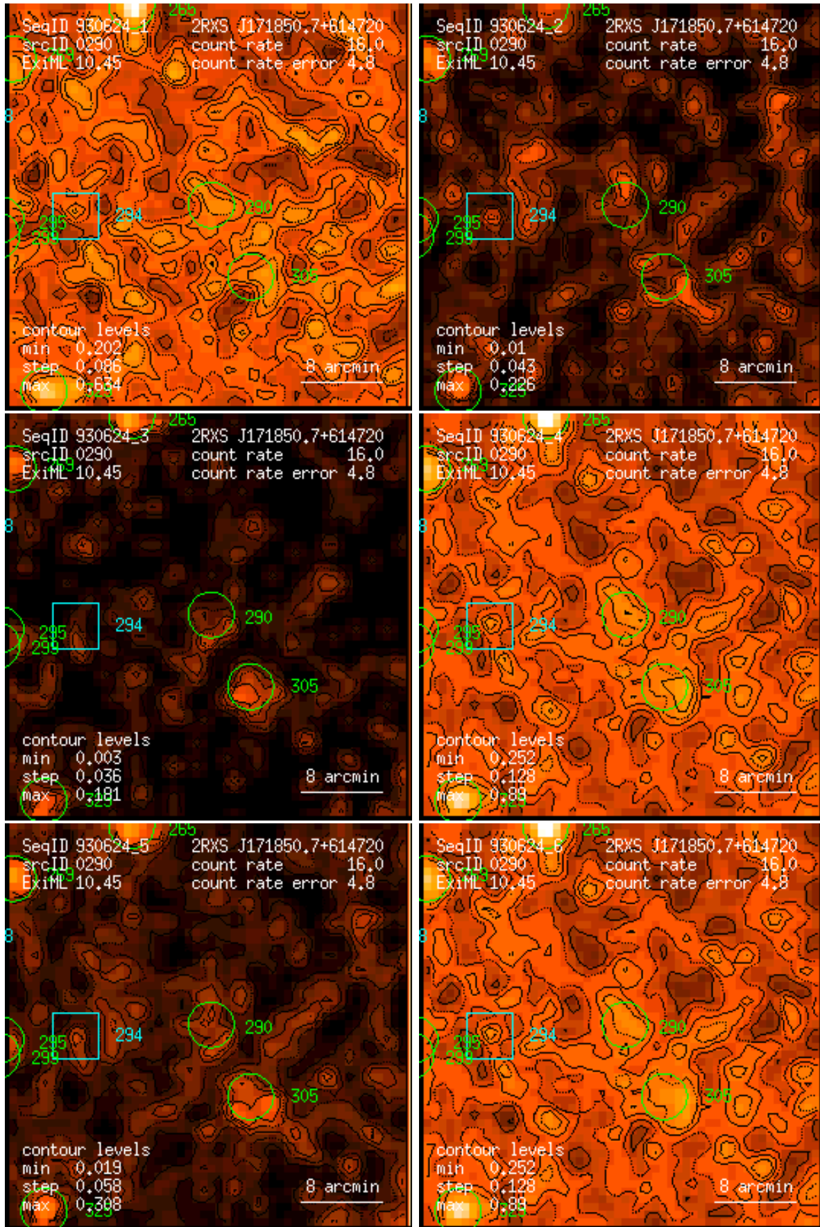
Figure 290: RASS 930624: detection 0290: band rate images, Gaussian filter: (1) PSPC channels 11 – 41, (2) 52 – 90, (3) 91 – 201, (4) 11 – 235, (5) 52 – 201, (6) 11 – 201. Broad band rates in counts/ks. Band rate contour levels in counts/ks/arcmin 2 .
