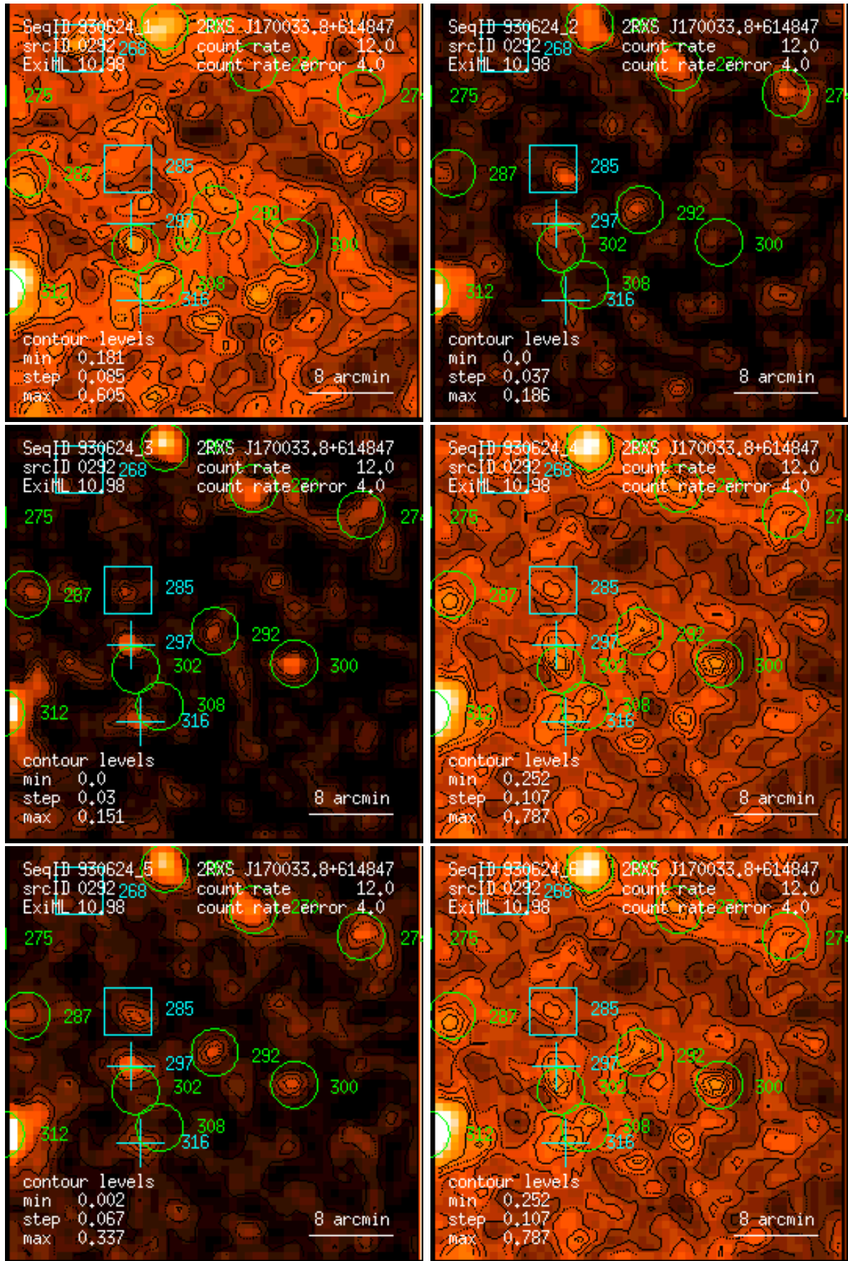
Figure 292: RASS 930624: detection 0292: band rate images, Gaussian filter: (1) PSPC channels 11 – 41, (2) 52 – 90, (3) 91 – 201, (4) 11 – 235, (5) 52 – 201, (6) 11 – 201. Broad band rates in counts/ks. Band rate contour levels in counts/ks/arcmin 2 .
