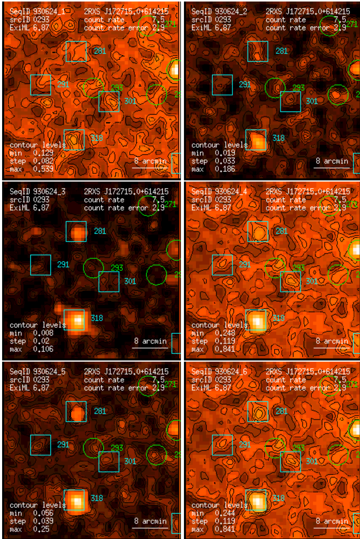
Figure 293: RASS 930624: detection 0293: band rate images, Gaussian filter: (1) PSPC channels 11 – 41, (2) 52 – 90, (3) 91 – 201, (4) 11 – 235, (5) 52 – 201, (6) 11 – 201. Broad band rates in counts/ks. Band rate contour levels in counts/ks/arcmin 2 .
